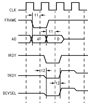
PCI Posted Write Cycles (fast decode)
