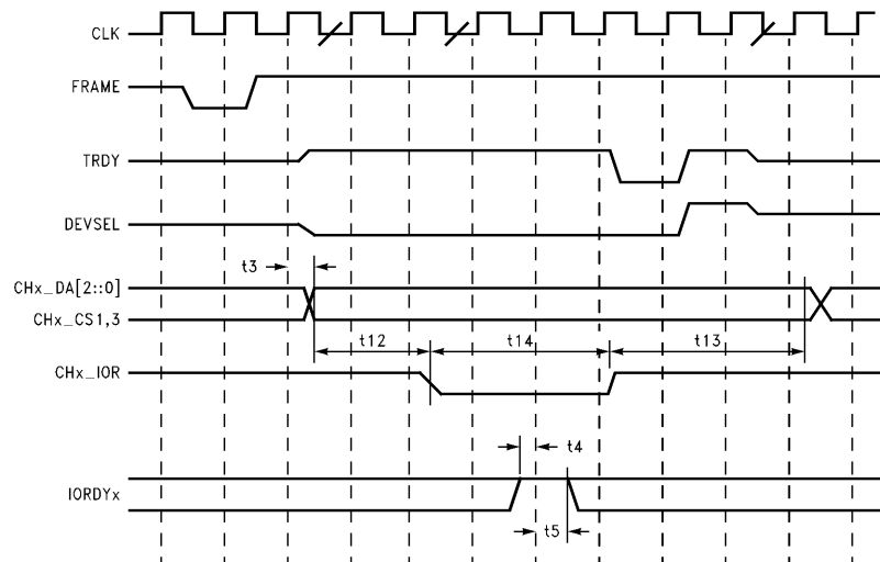
IDE Non Data Cycles (read or write)
