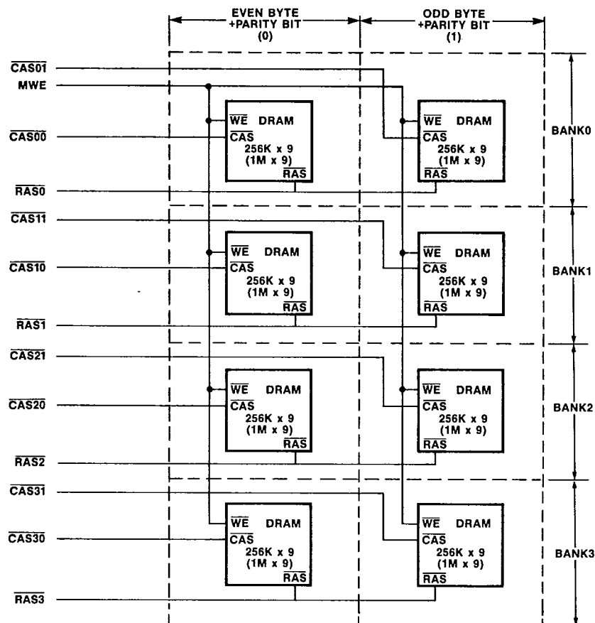
Figure 2.5 DRAM Organization
