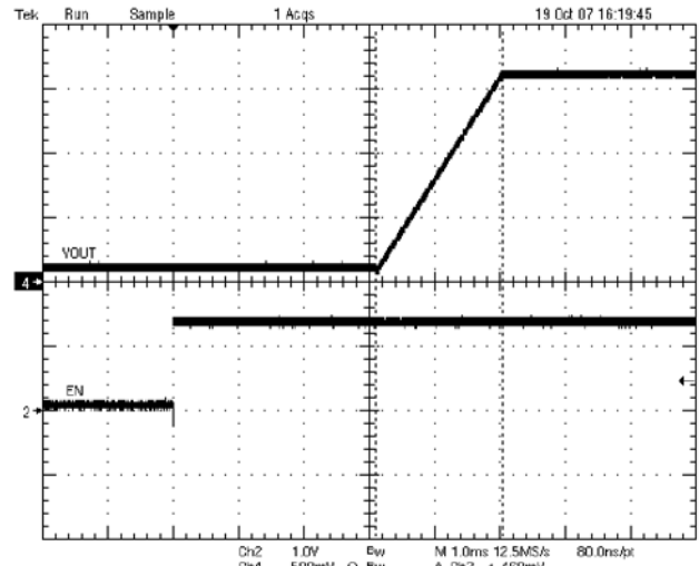
Figure 10. AMD Startup
