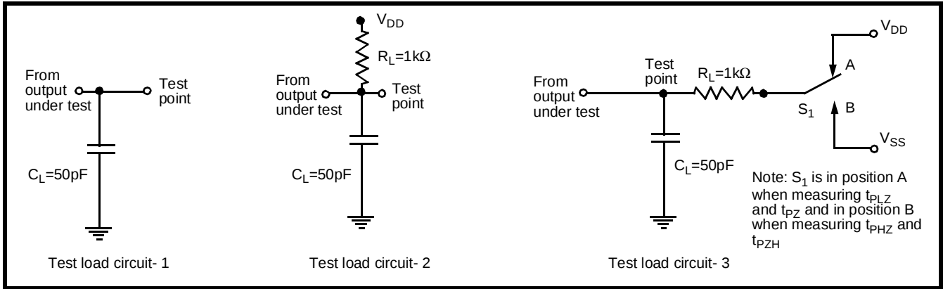
Figure 17 - Test Load Circuits
