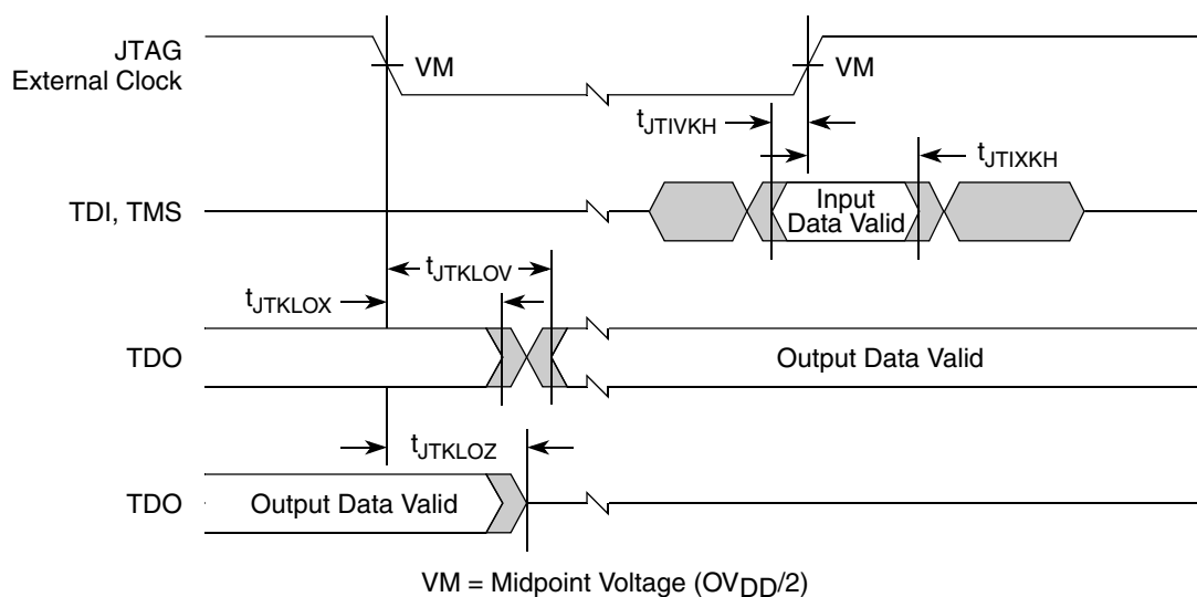
Figure 28. Test Access Port Timing Diagram
