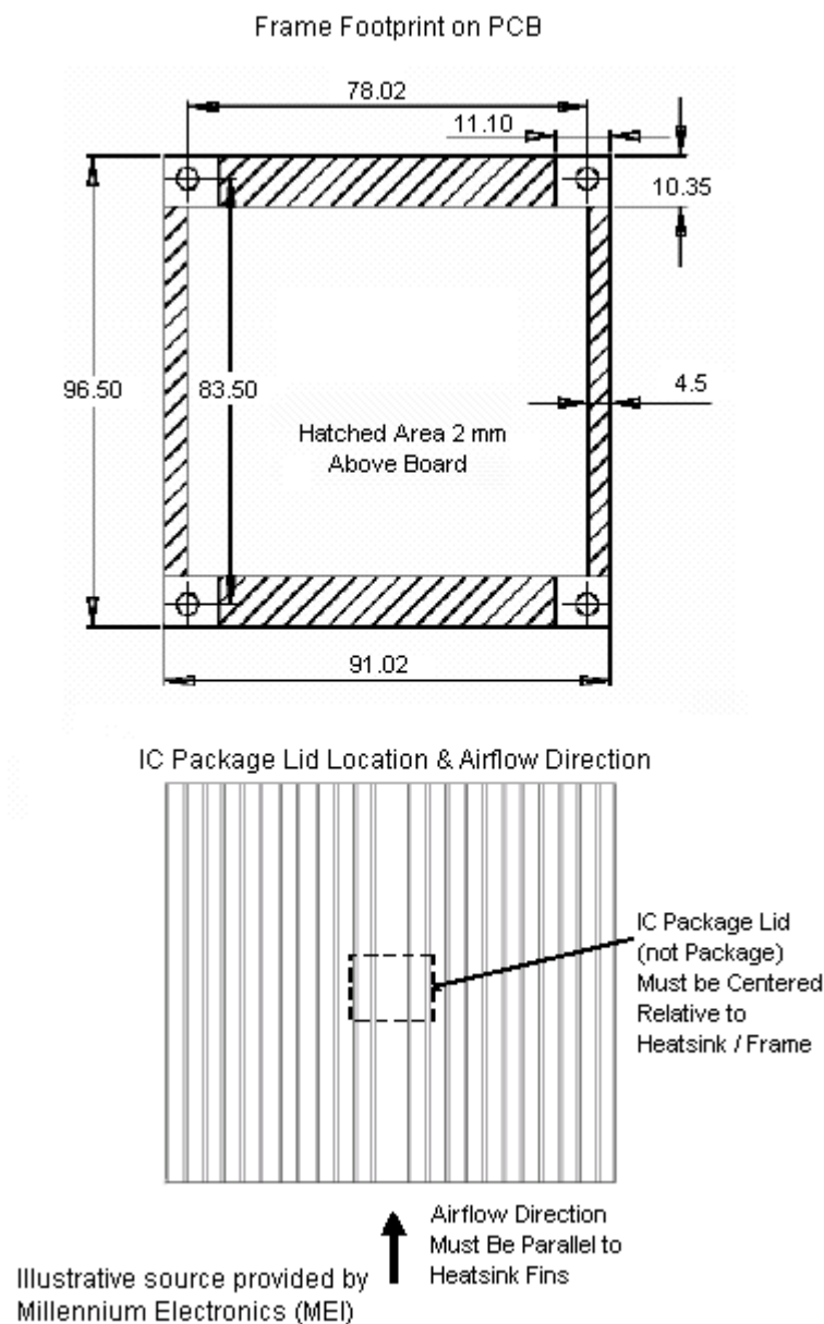
Figure 49. Exploded Views (1) of a Heat Sink Attachment using a Plastic Force
