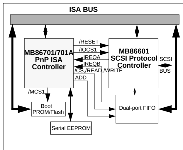
Figure 6. Typical MB86701/701A Application - SCSI Controller
