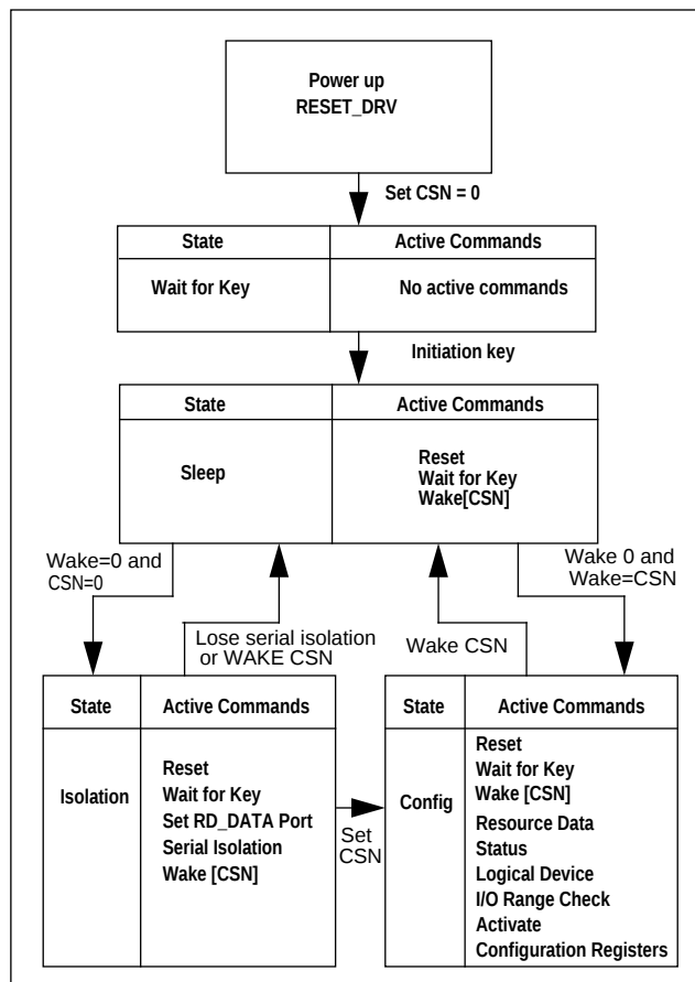
Figure 1. Plug and Play Configuration Process States
