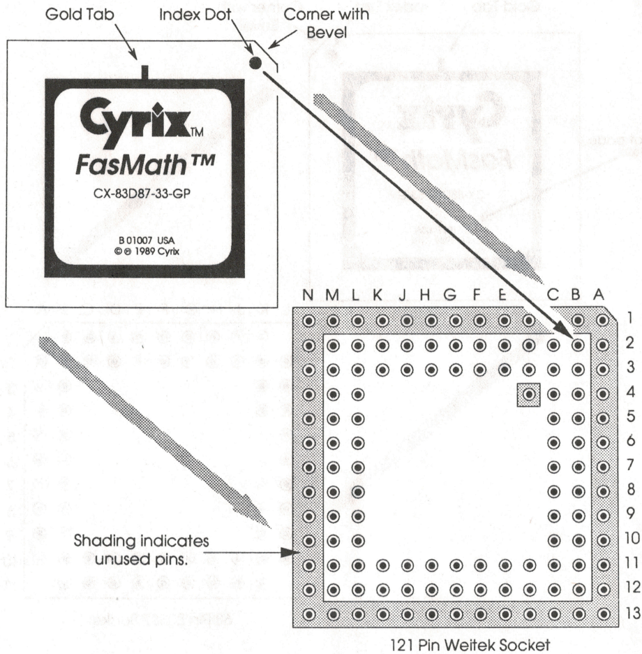
Figure 3(a). Installation Orientation for 121 Pin Socket.
