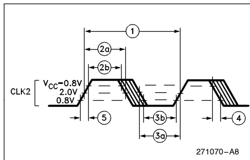
Figure 67. CLK2 Timing
