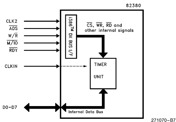
Figure 1. Translation of i386™ DX Signals to Internal M82380 Timer Unit Signals
