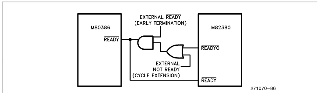
Figure 53. External 'READY' Control Logic
