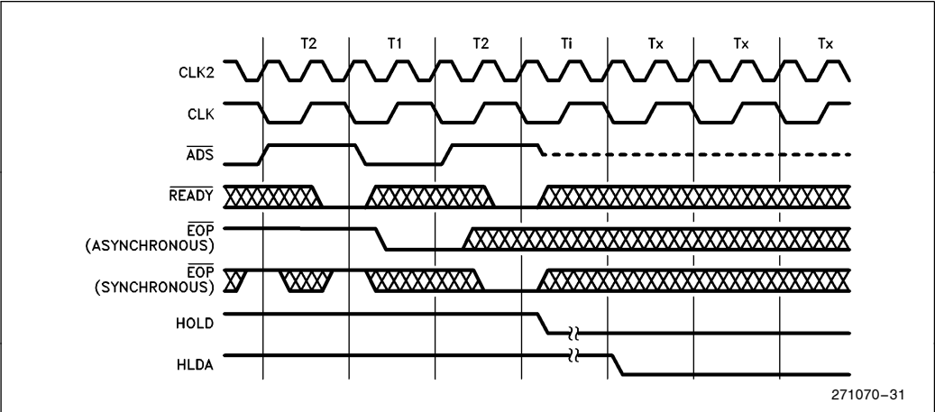
Figure 32. Termination of a DMA Process Due to an External \overline{EOP}
