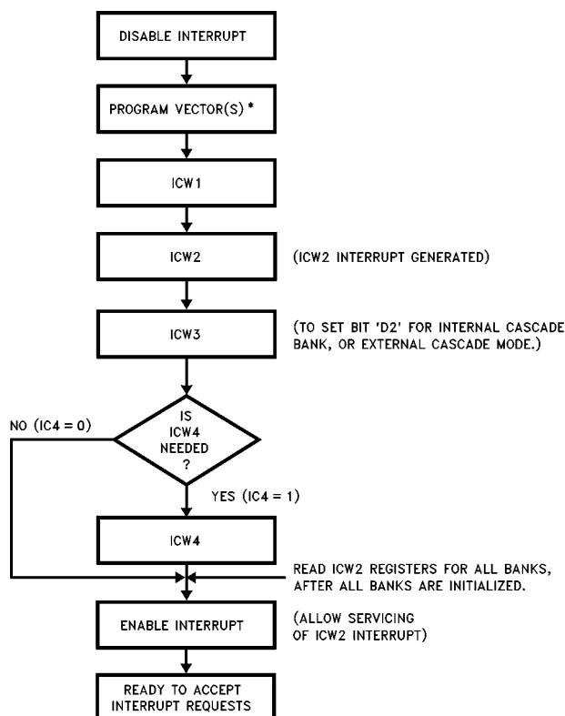
Figure 42. Initialization Sequence
