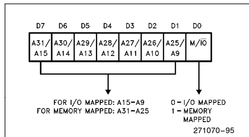
Figure 59. Relocation Register
