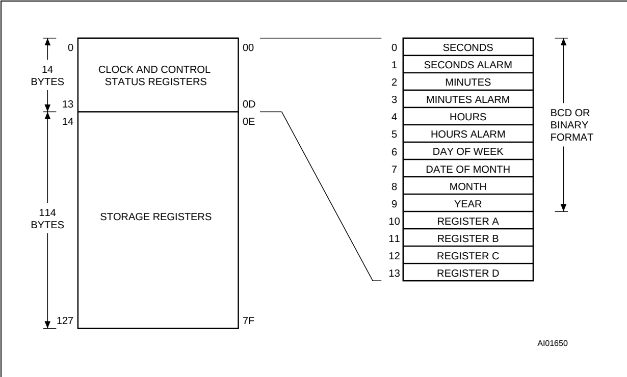
Figure 11. Address Map
