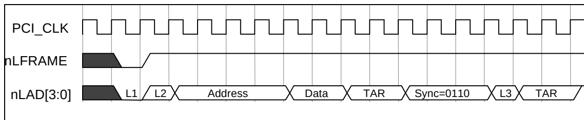
FIGURE 8 – I/O WRITE
