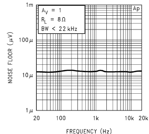
Noise Floor
