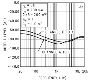
Channel Separation
