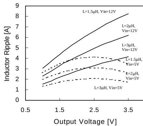
Figure 12 – Inductor ripple current vs. Vout
