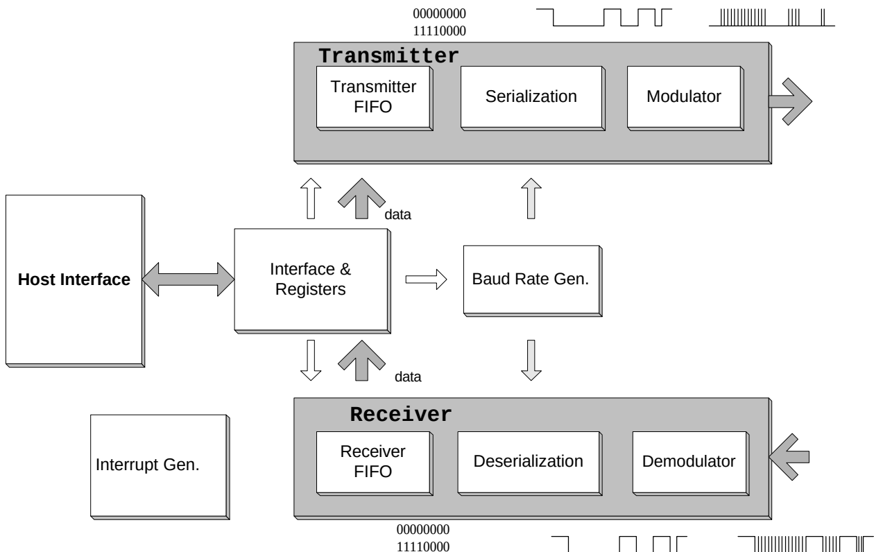
Figure 10-11. CIR Block Diagram
