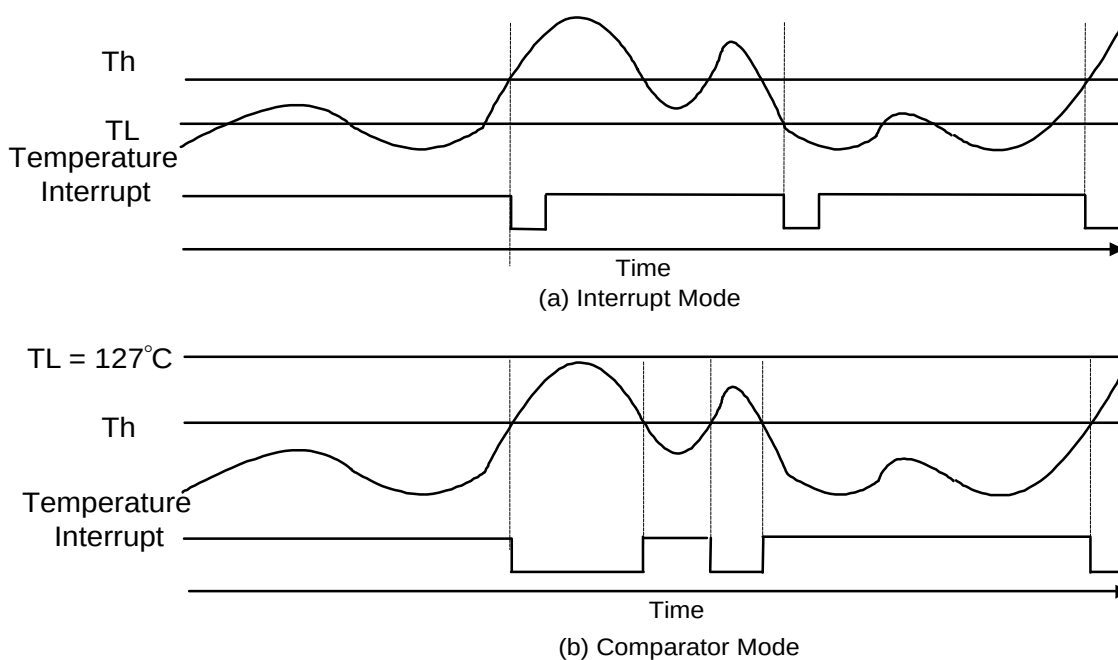
Figure 10-5. Temperature Interrupt Response Diagram
