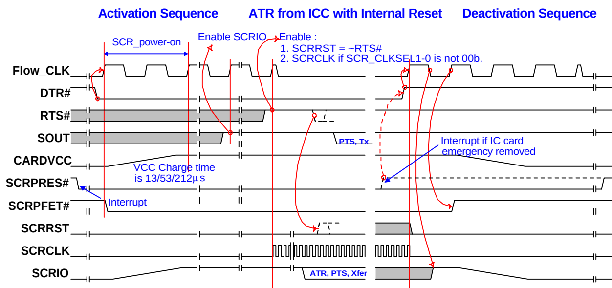
Figure 10-9. Waveform Example of IFD
