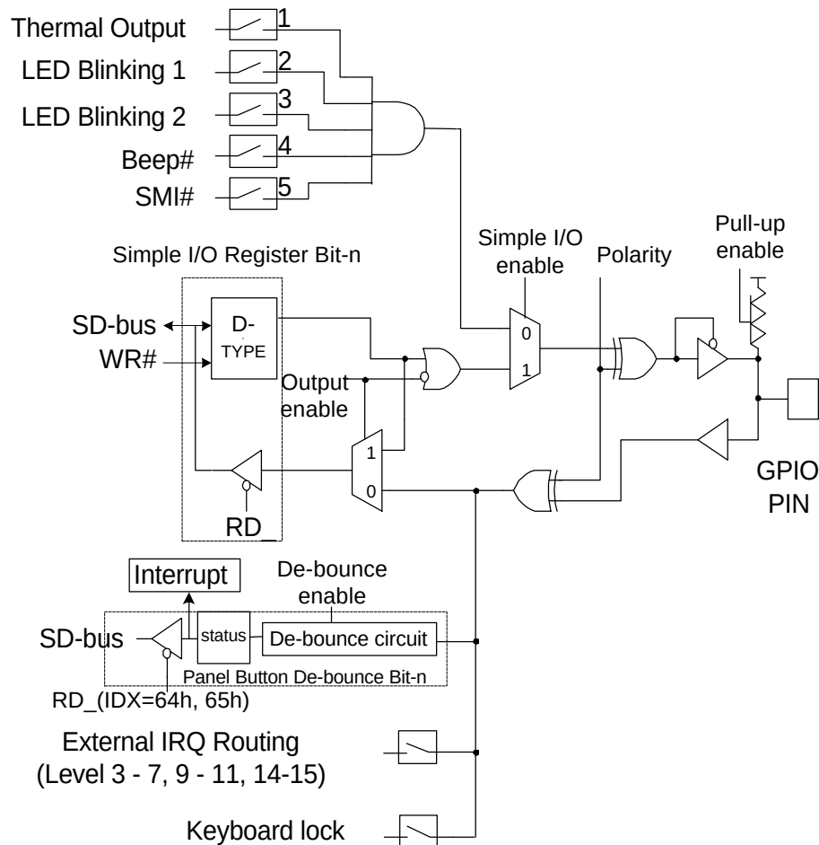
Figure 10-3. General Logic of GPIO Function
