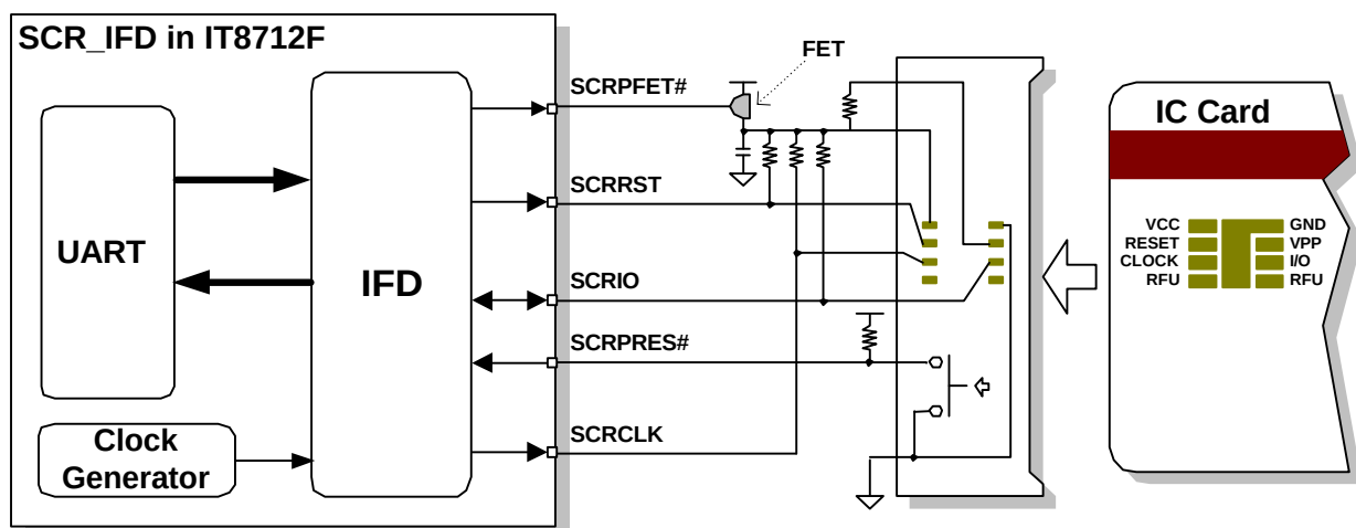
Figure 10-7. Smart Card Reader Application
