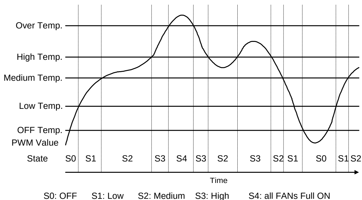
Figure 10-6. SmartGuardian Automatic Mode
