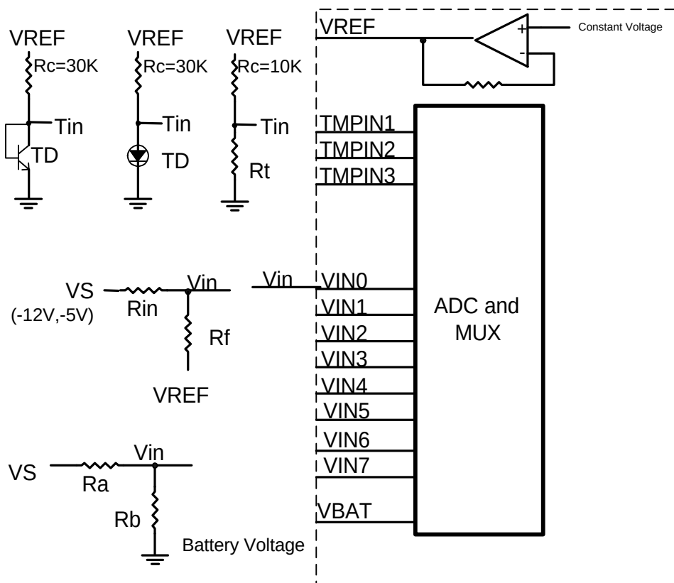
Figure 10-4. Application Example. Resistor should provide approximately 2V at the Analog Inputs.
