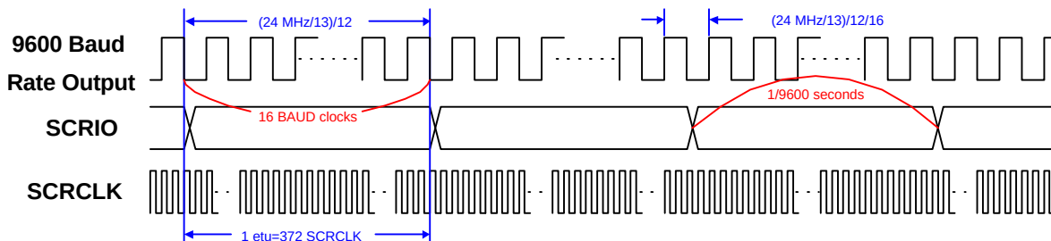
Figure 10-8. 9600 Baud Rate Example
