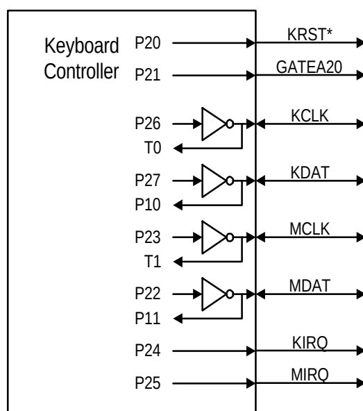
Figure 10-10. Keyboard and Mouse Interface
