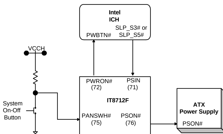
Figure 8-1. IT8712F Special Applications Circuitry for Intel ICH
