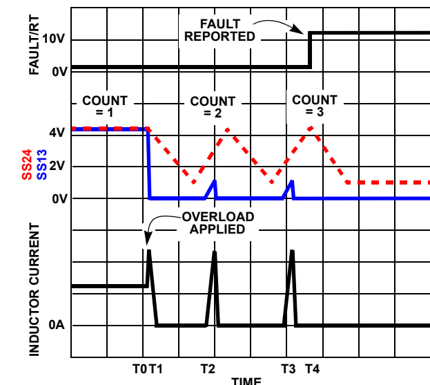
FIGURE 8. OVERCURRENT OPERATION
