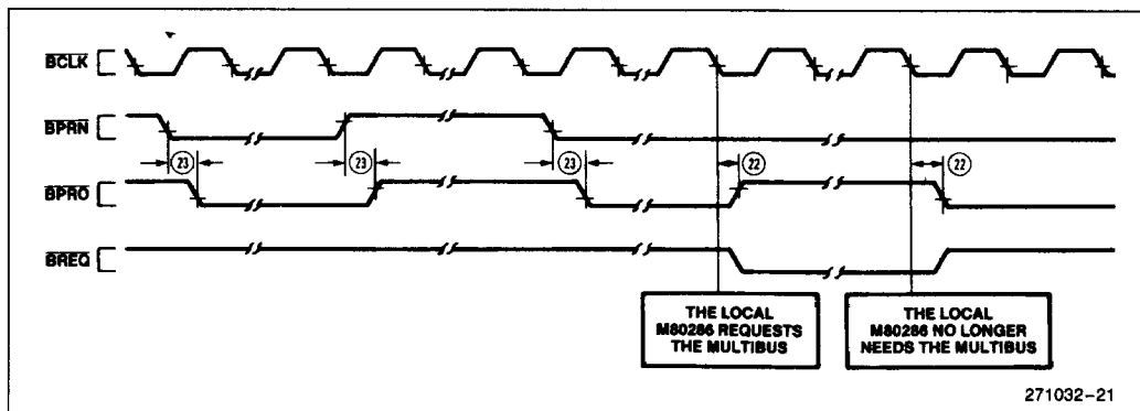
Figure 17. \bar{B}\bar{P}\bar{R}\bar{N} to \bar{B}\bar{P}\bar{R}\bar{O} Timing Relationship
