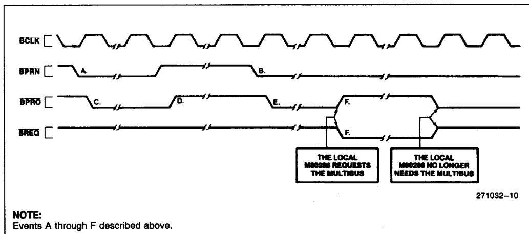
Figure 10. Serial Priority Bus Behavior
