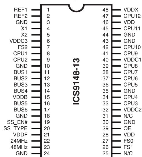
48-Pin SSOP
