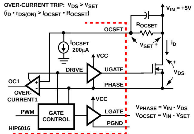
FIGURE 9. OVER-CURRENT DETECTION
