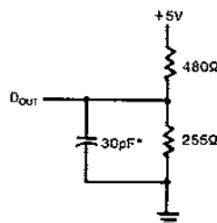
Figure 1 Output Load
