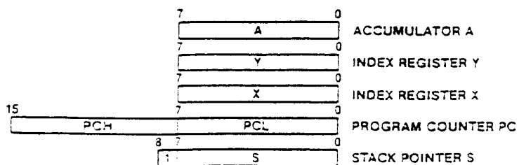
Figure 3. Microprocessor Programming Model
