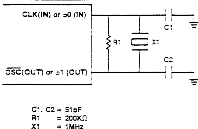
Figure 2(a). Crystal Circuit for Internal Oscillator
