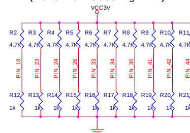
(Power On Setting Pin)
