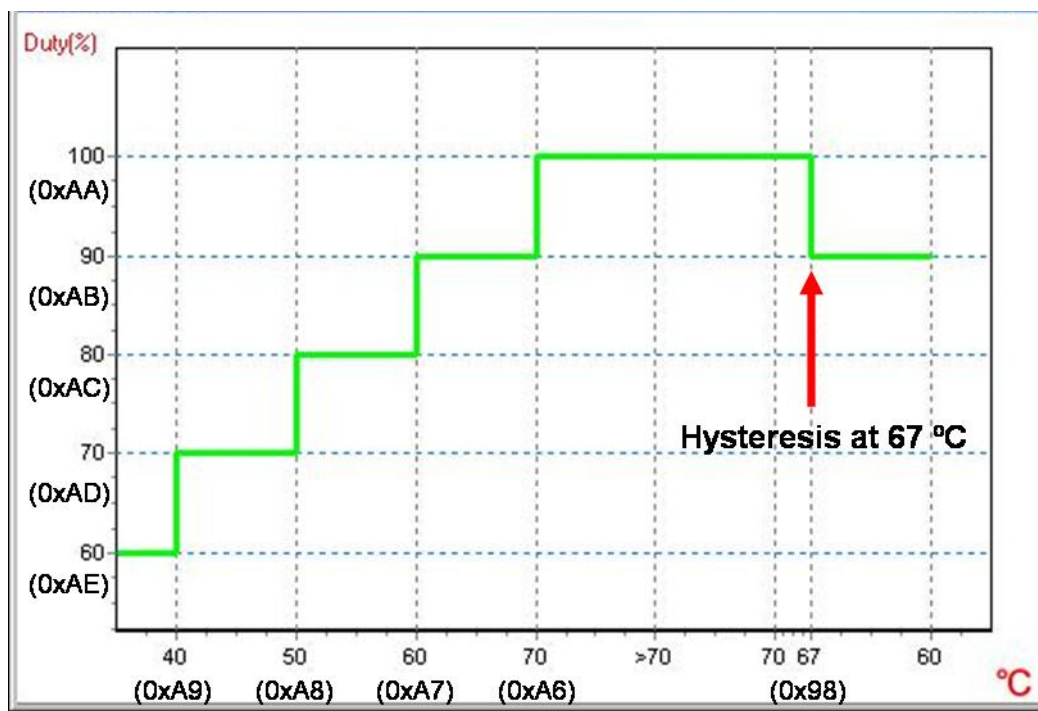
Figure 8 Stage mode fan control illustration-2
