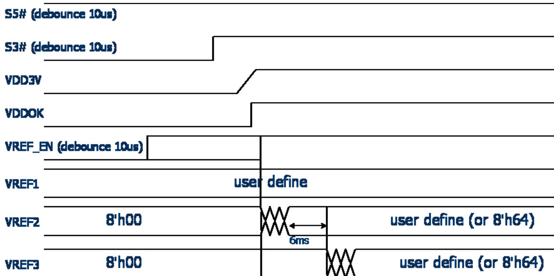
Figure 22 VREF timing: S3→S0
