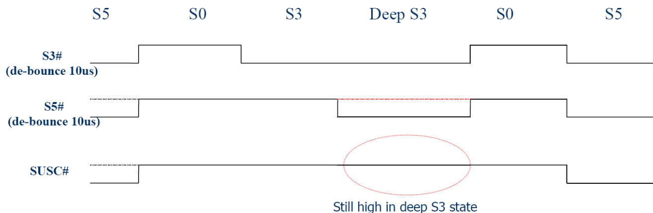
Figure 25 SUSC# timing
