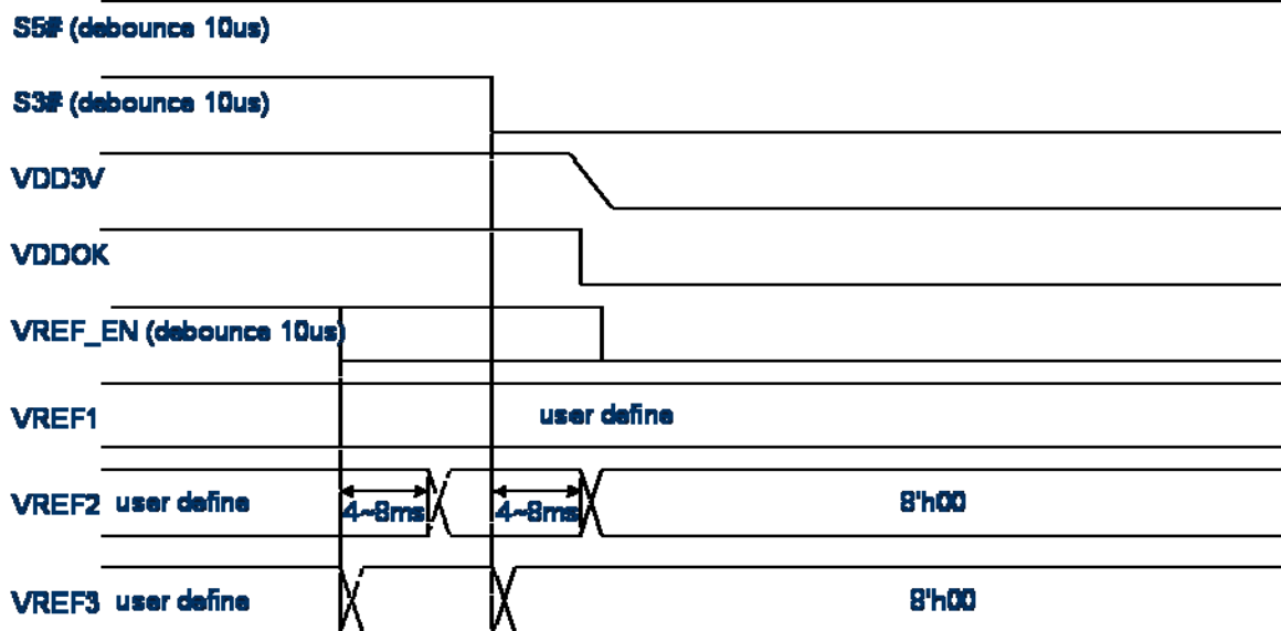
Figure 21 VREF timing: S0→S3
