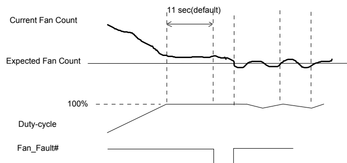
Figure 17 FAN_FAULT# event
