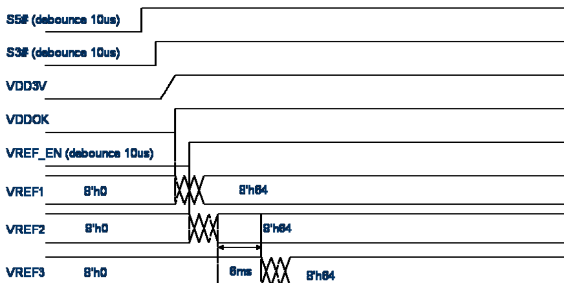
Figure 20 VREF timing: S5→S0
