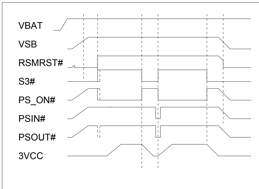
Figure 19 Optional timing: Always on
