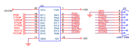
UART 2 PORT INTERFACE
