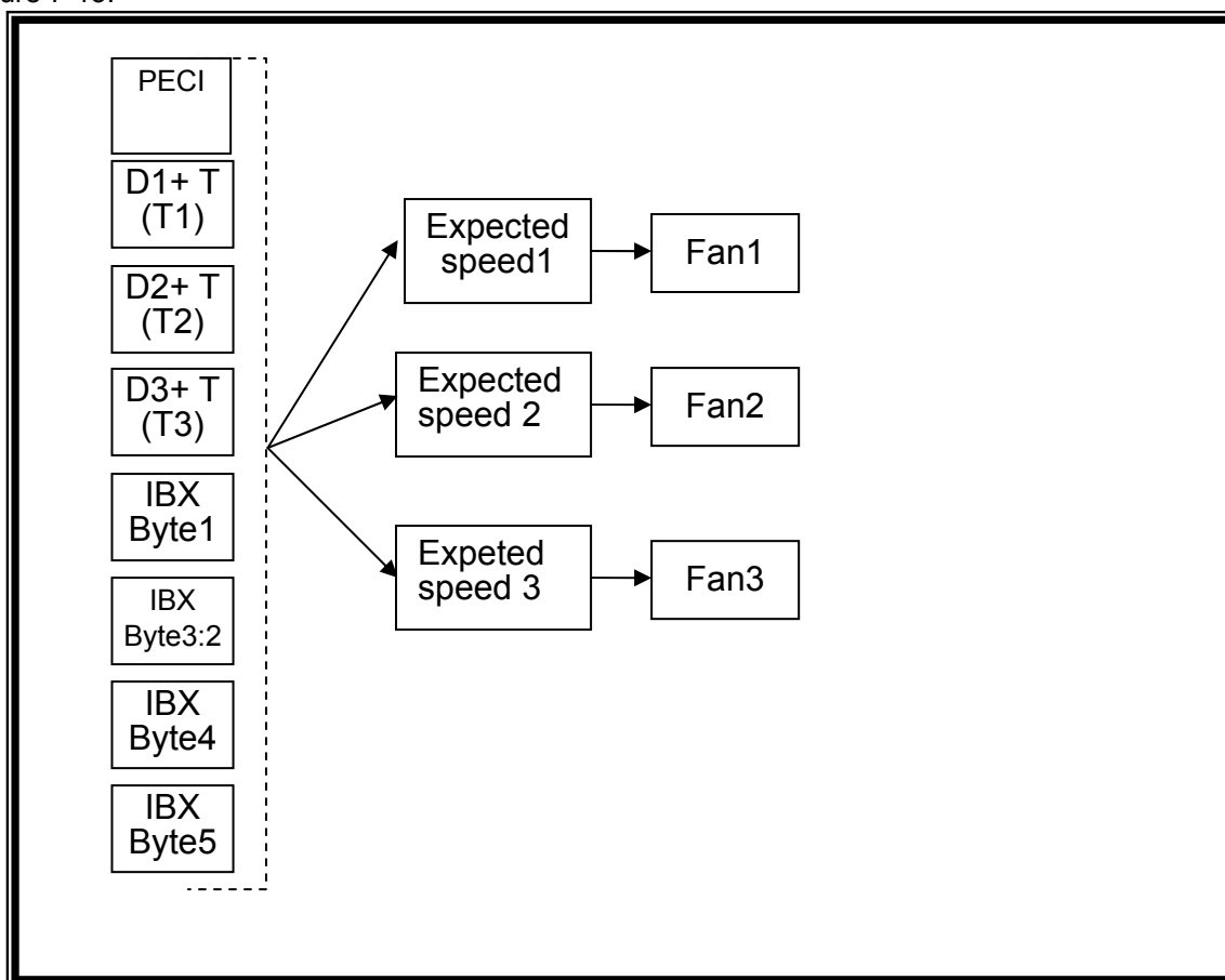
Figure 13 Relative temperature fan control
