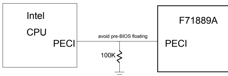
INTEL PECI Typical Application
