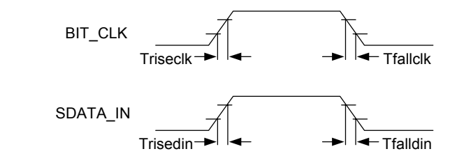
Signal Rise and Fall timing diagram
