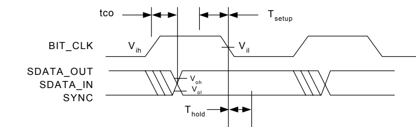
Data Output and Input timing diagram
