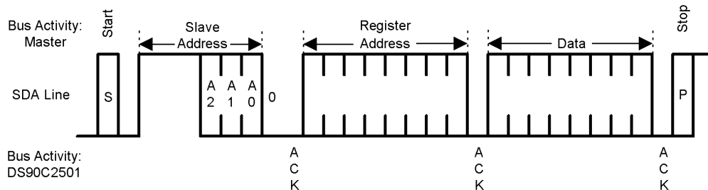
FIGURE 13. Byte Write
