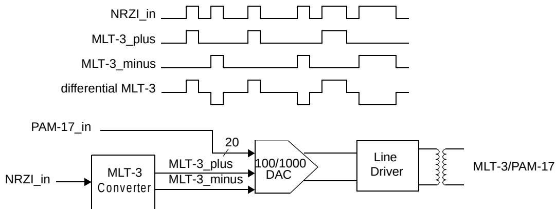
Figure 11. NRZI to MLT-3 Conversion
