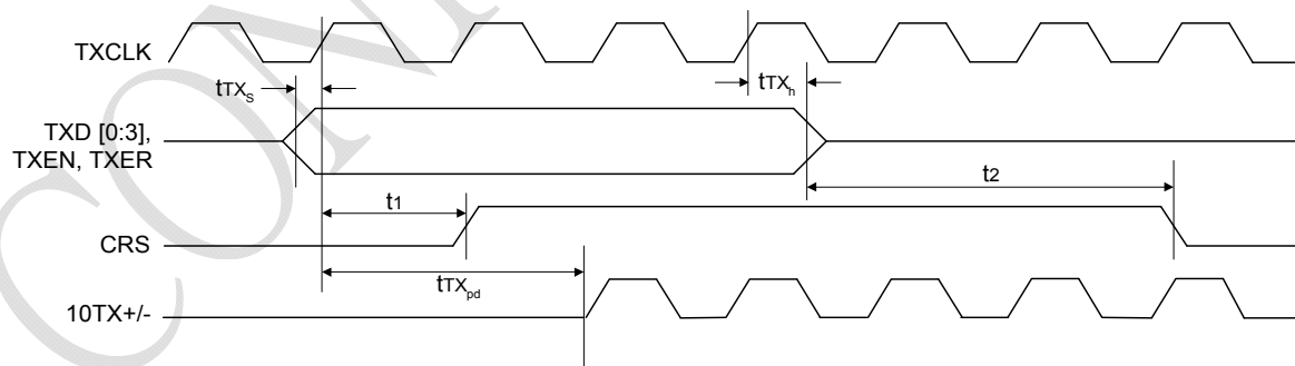
9.4.12 MII 10BASE-T Nibble Transmit Timing Diagram
