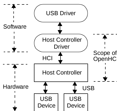
Figure 4. USB System Domains
