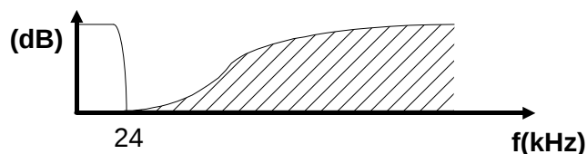
Figure 24. Modulator Output Spectrum
