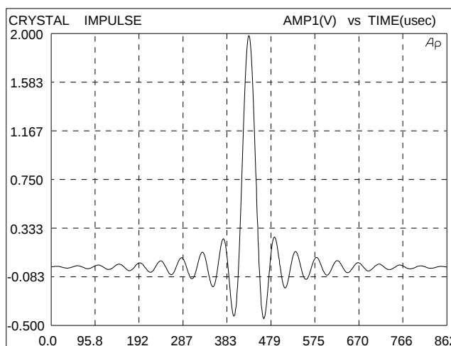
Figure 14. Impulse Response
