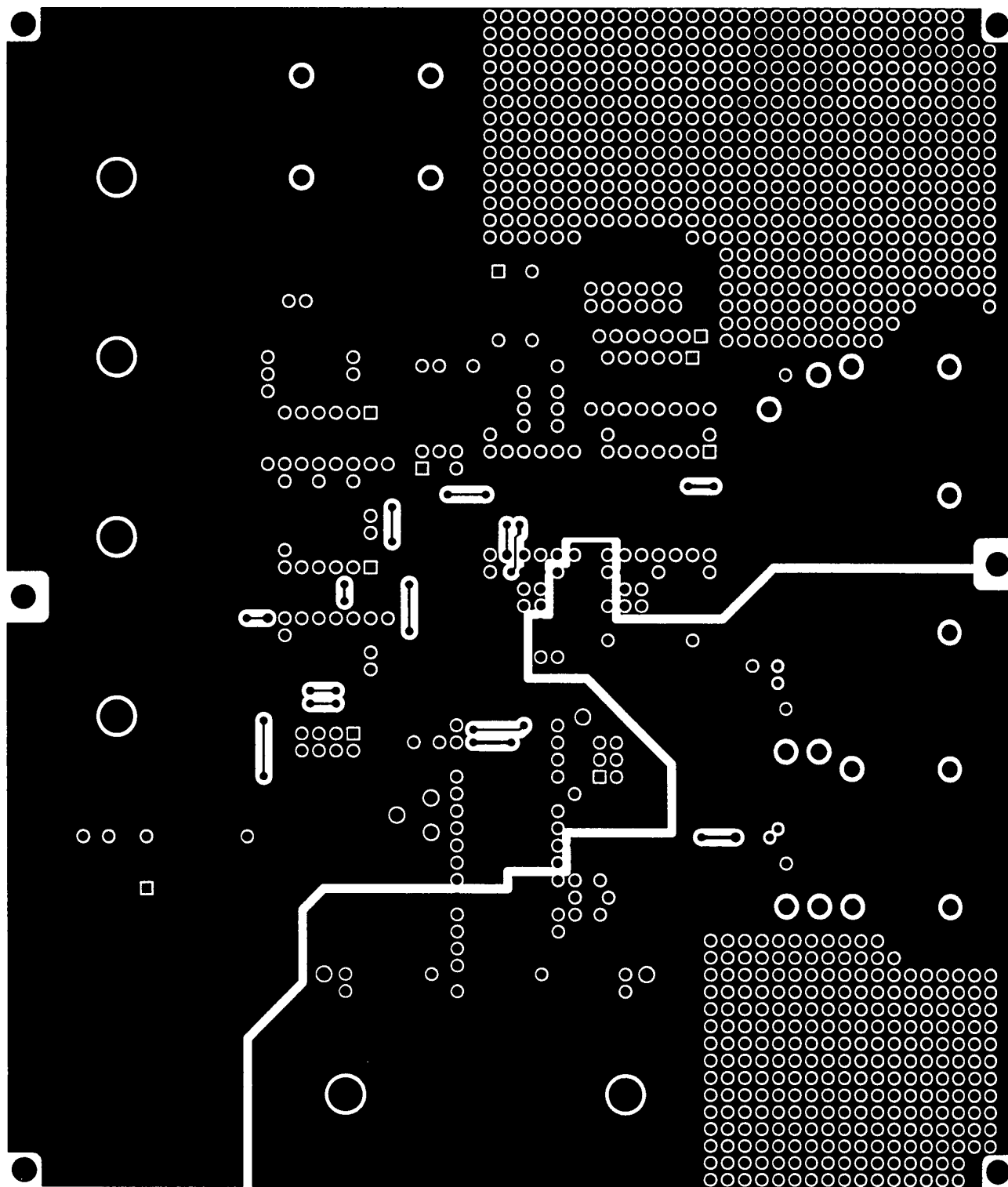
Figure 4. Top Ground Plane Layer (NOT TO SCALE)
