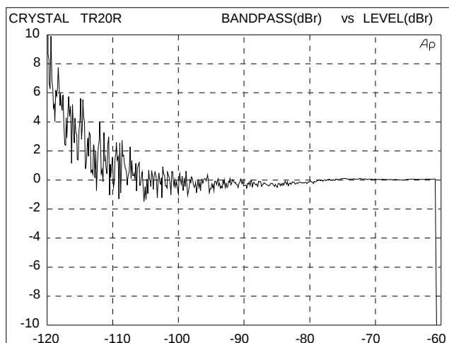
Figure 13. Fade-to-Noise Linearity
