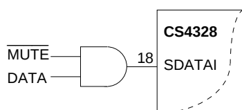
Figure 8. -120 dB Muting
