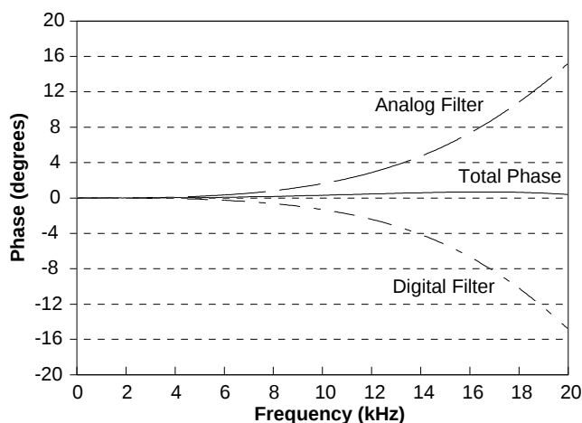
Figure 27. Deviation From Linear Phase
