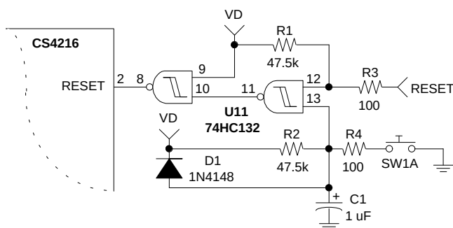
Figure 6. Reset Circuit
