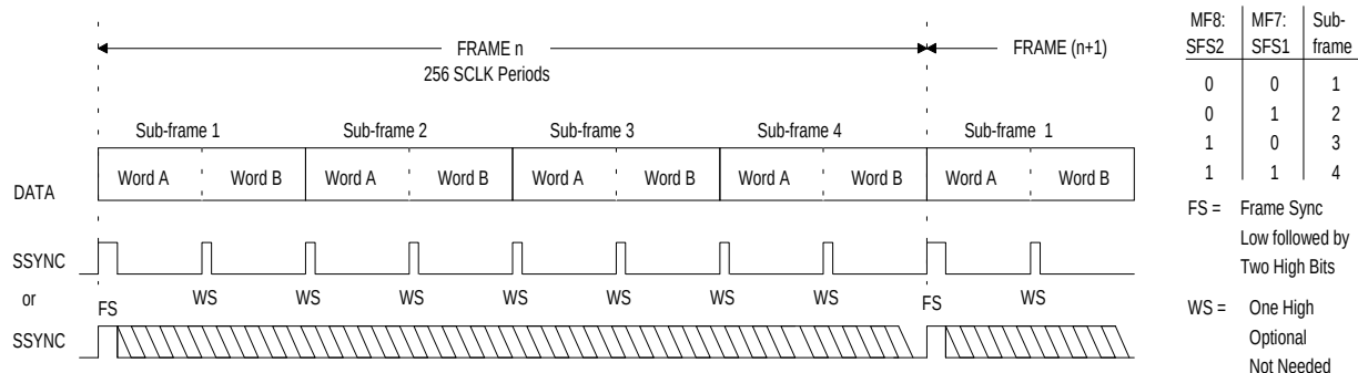
Figure 7. SM1, SM2 - 256 Bits per Frame.
