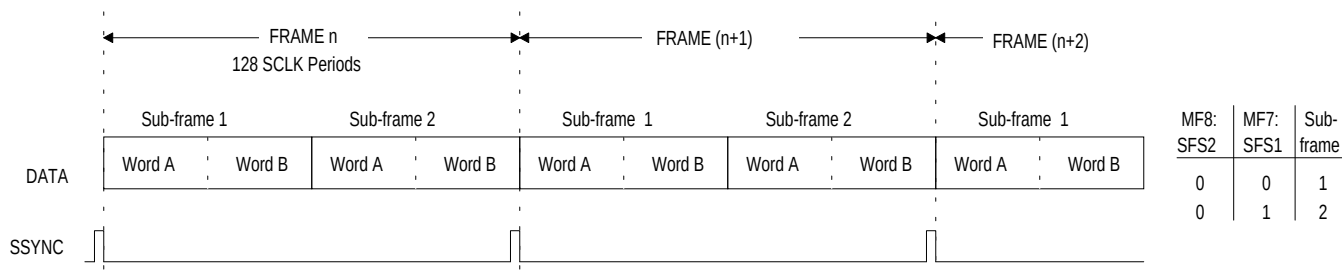
Figure 11. SM3-Slave - 128 BPF; \text{MF1:F1} , \text{MF2:F2} = 01
