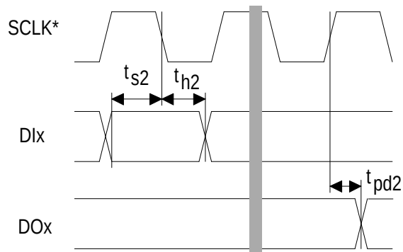
DI/DO Timing
