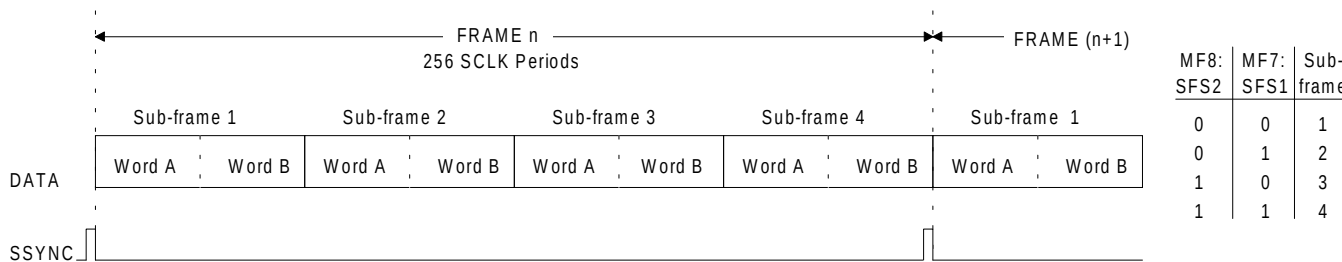
Figure 12. SM3-Slave - 256 BPF; \text{MF1:F1} , \text{MF2:F2} = 10
