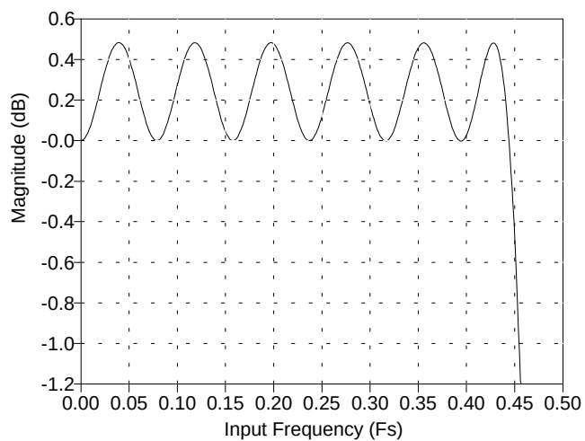
Figure 22. CS4216 ADC Passband Ripple
