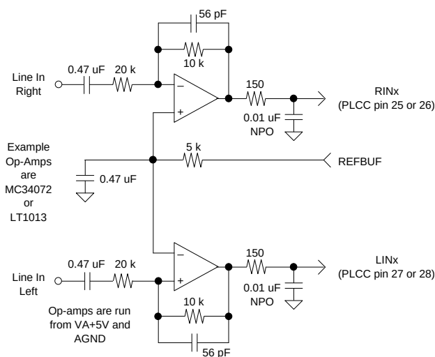
Figure 2. DC Coupled Input.
