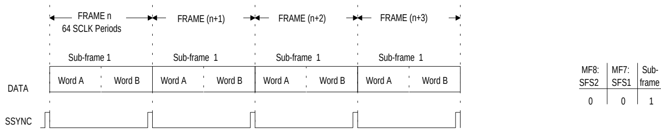
Figure 10. SM3-Slave - 64 BPF; \text{MF1:F1} , \text{MF2:F2} = 00
