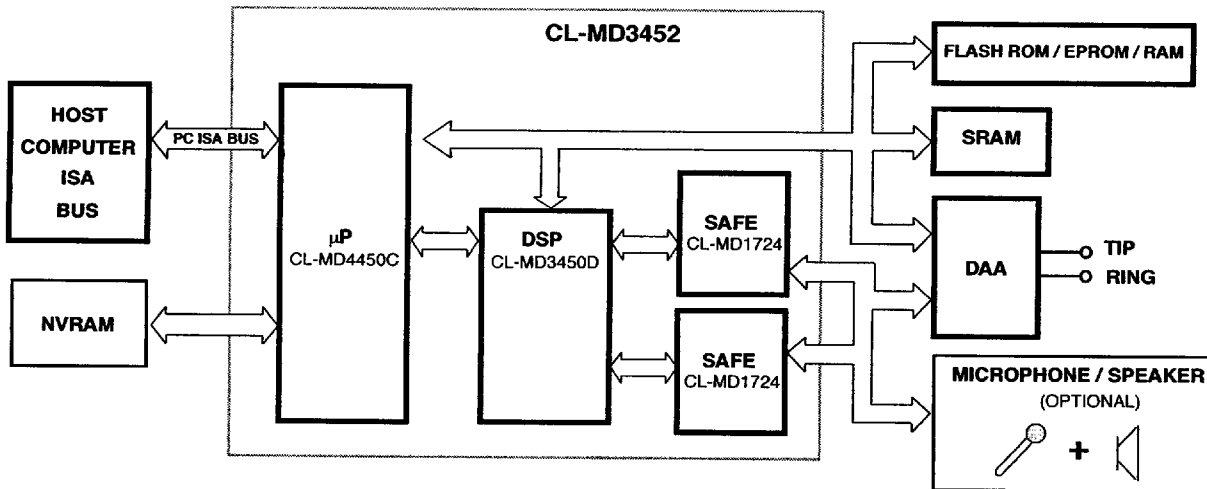
Figure 1-3. CL-MD3452 Functional Block Diagram
