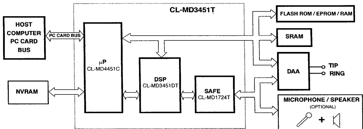
Figure 1-5. CL-MD3451T PC Card Functional Block Diagram
