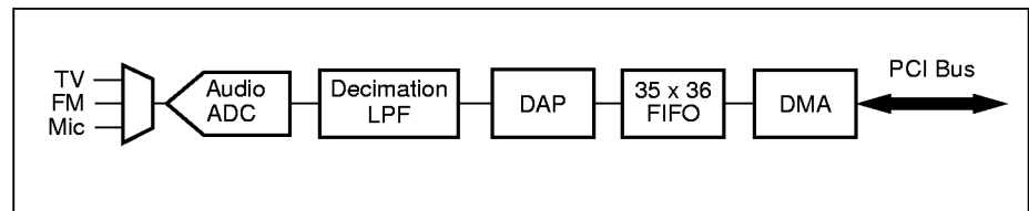
Figure 29. Audio Data Path
