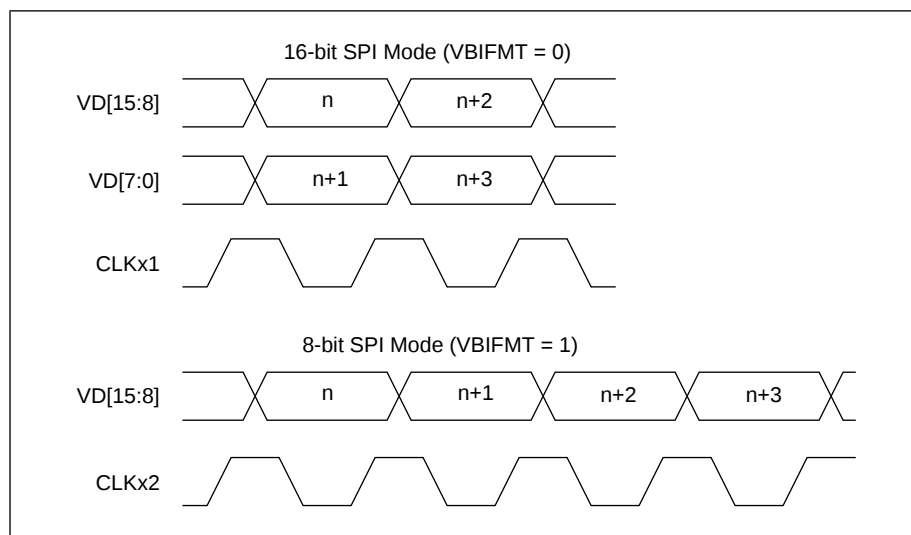
Figure 1-22. VBI Sample Ordering
