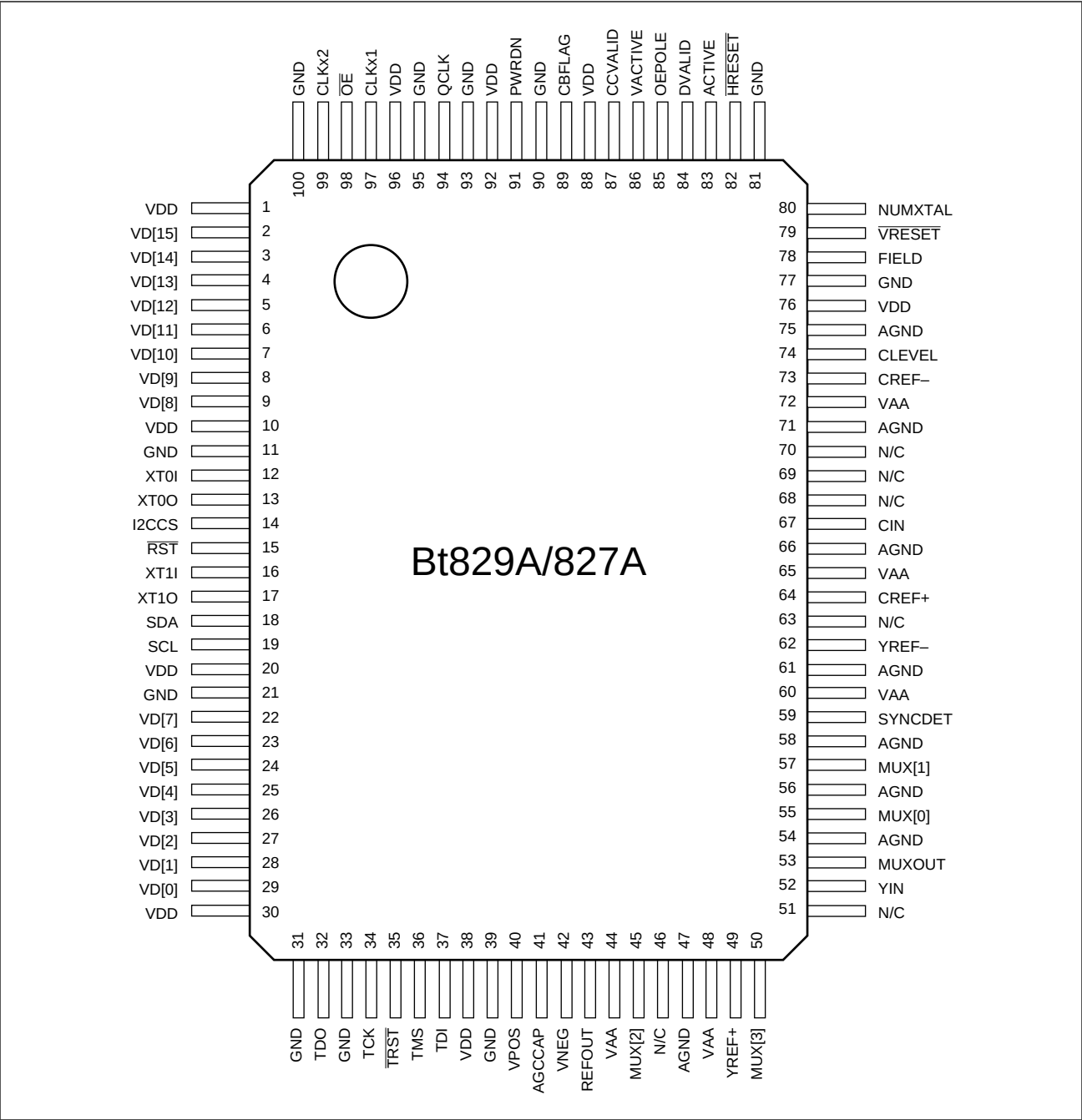
Figure 2. Bt829A/7A Pinout
