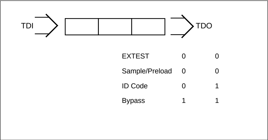
Figure 41. Instruction Register
