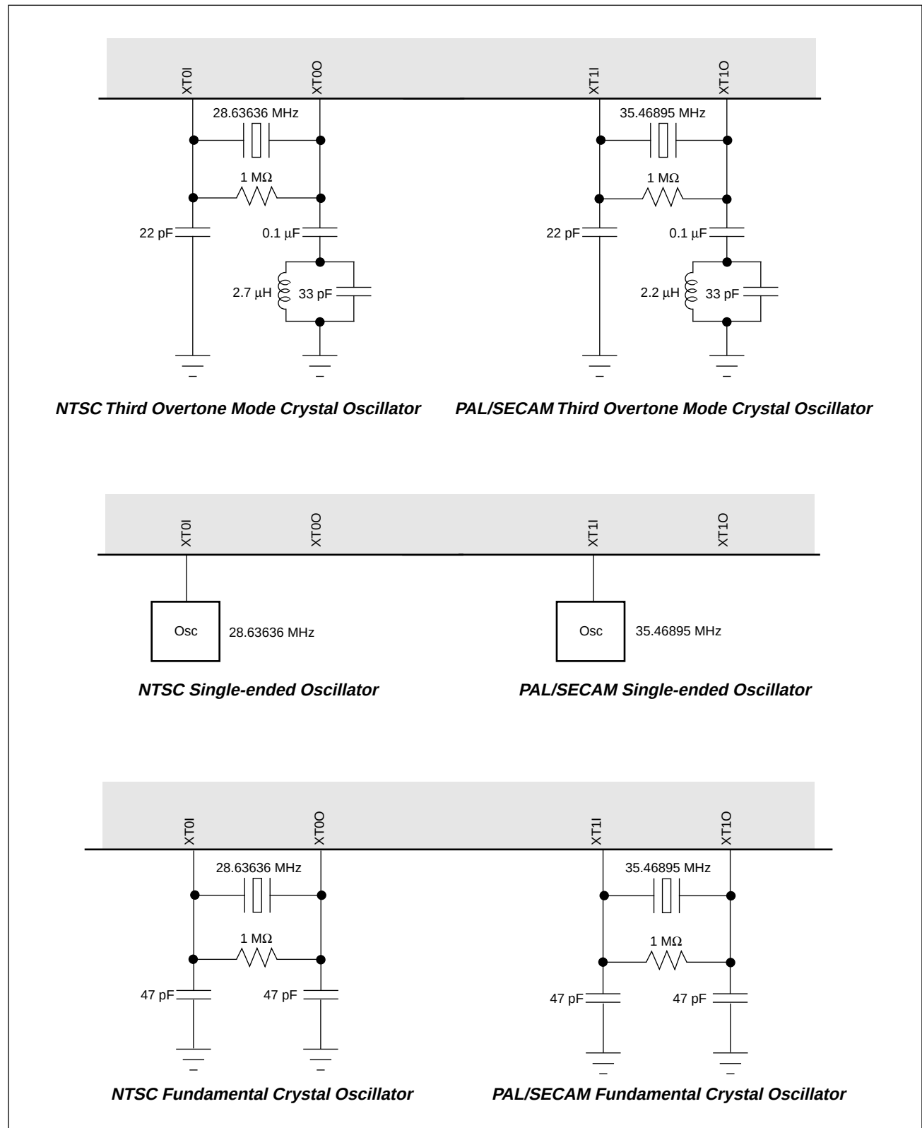
Figure 29. Clock Options
