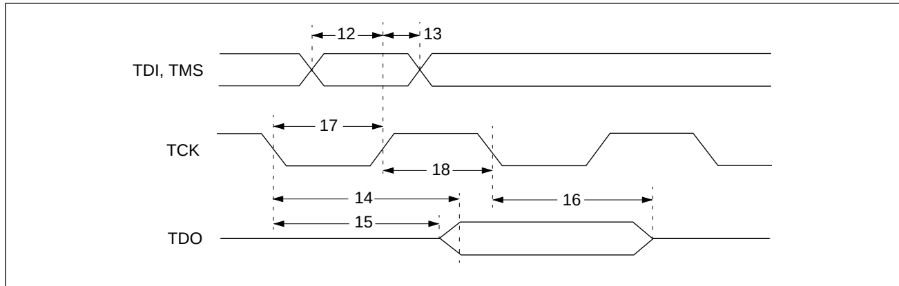
Figure 50. JTAG Timing Diagram
