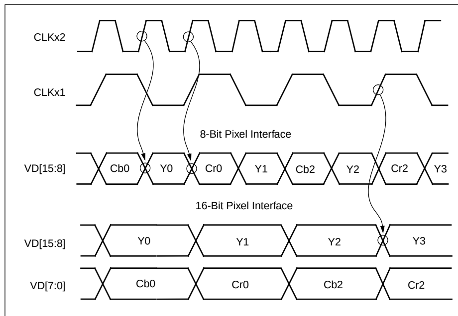
Figure 32. YCrCb 4:2:2 Pixel Stream Format (SPI Mode, 8 and 16 Bits)
