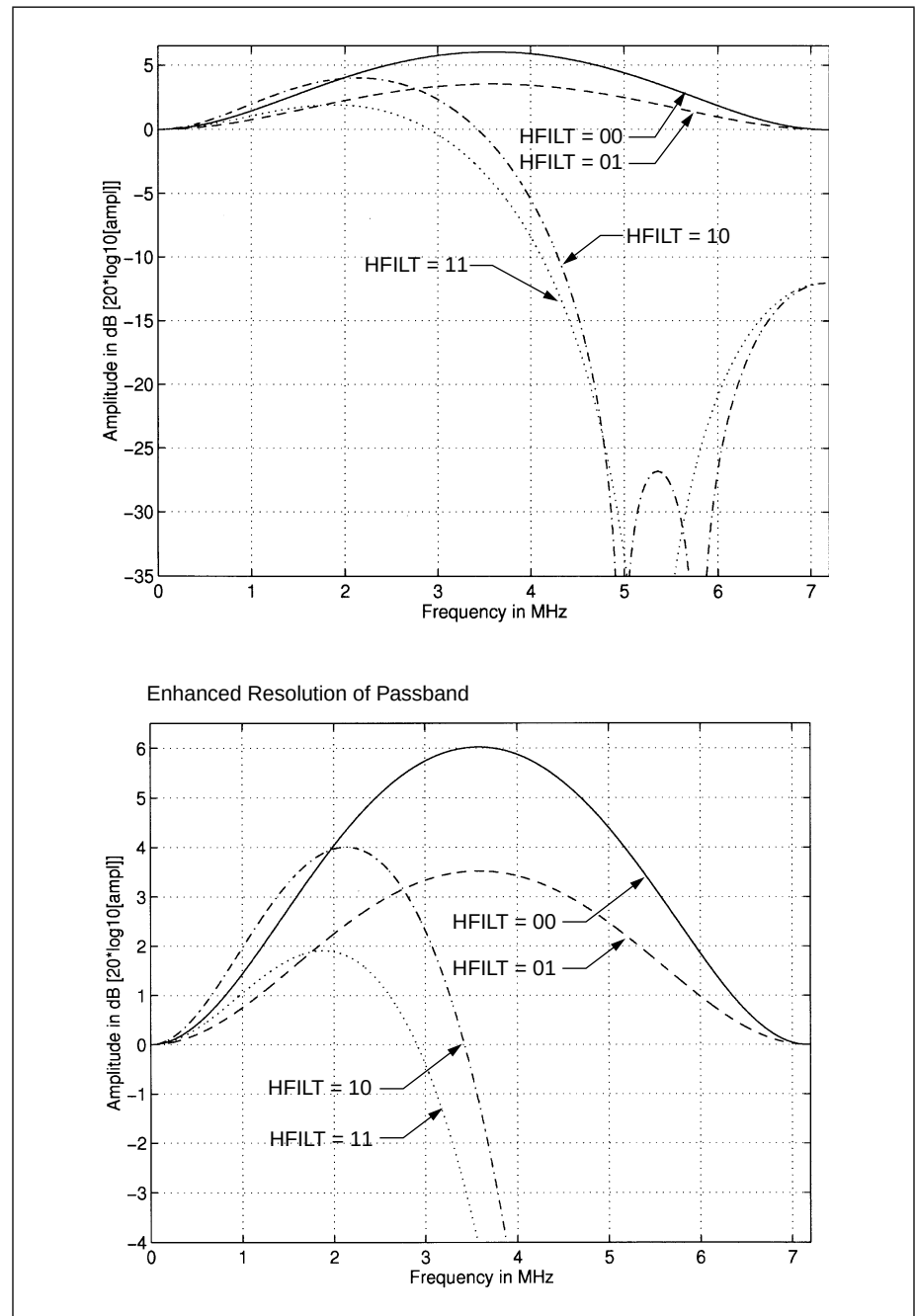
Figure 12. Peaking Filters
