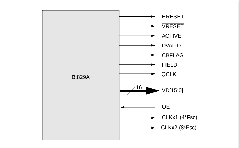
Figure 33. Bt829A/827A Synchronous Pixel Interface, Mode 1 (SPI-1)
