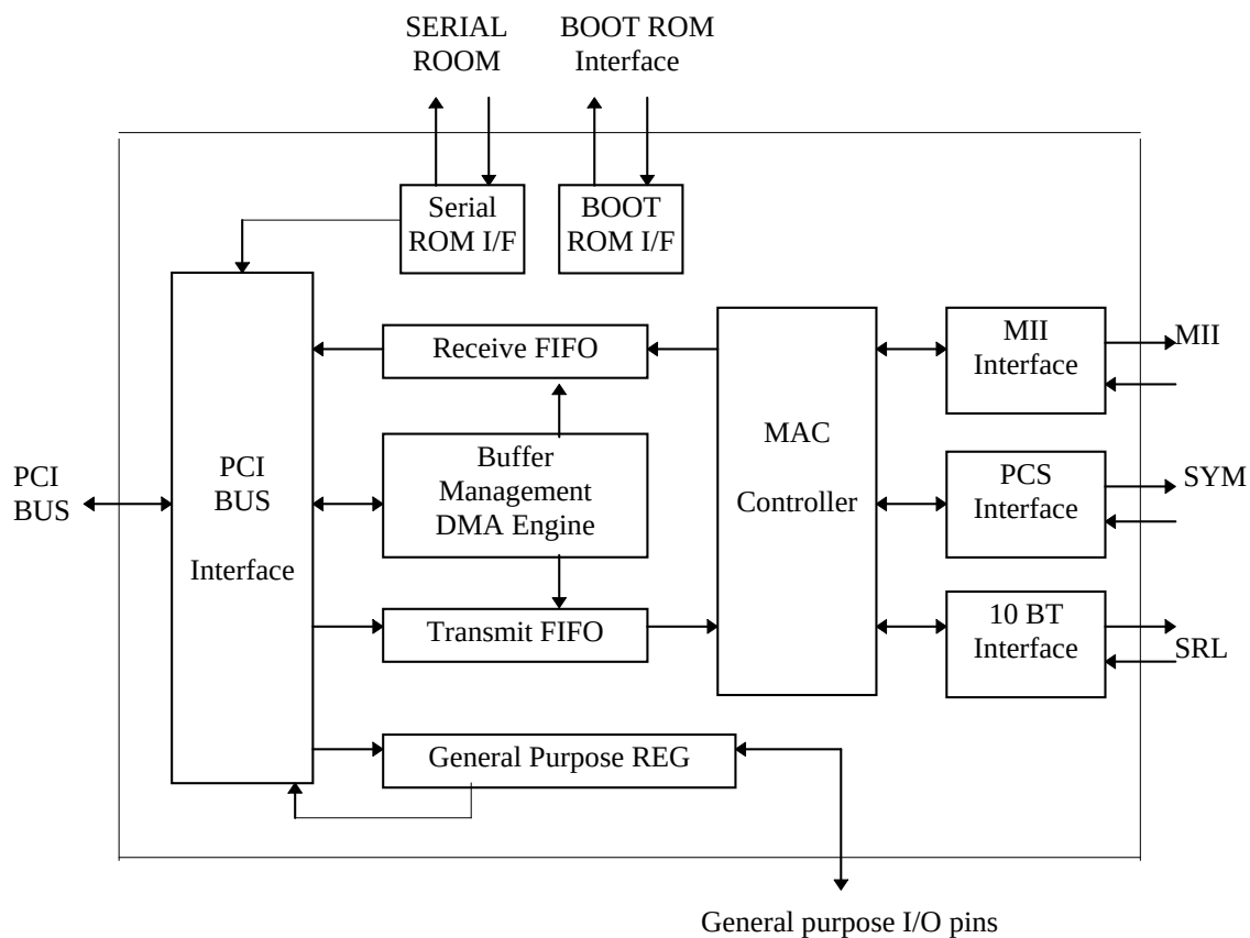
Fig - 1 AX88140A Block Diagram
