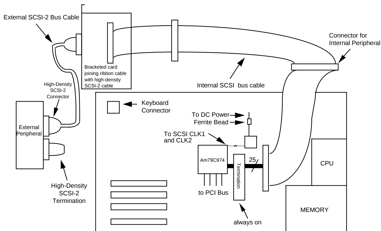
Figure E-3. Motherboard Layout — Approach #1
