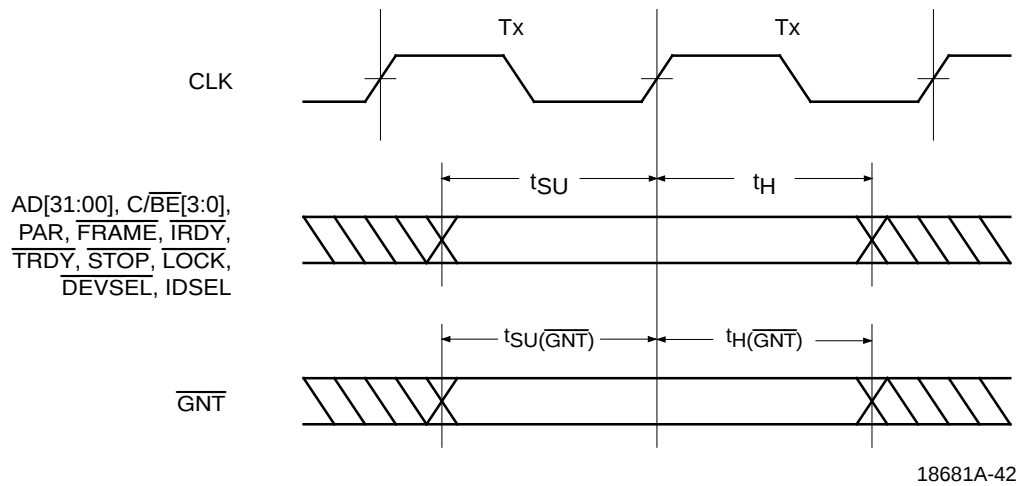
Input Setup and Hold Timing
