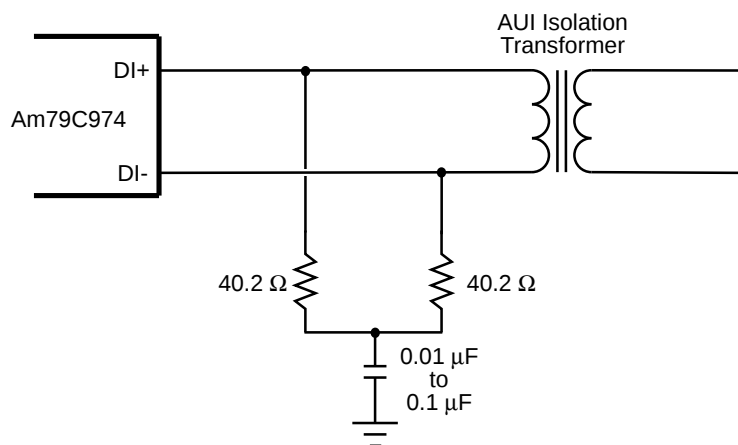
Figure 20. Differential Input Termination
