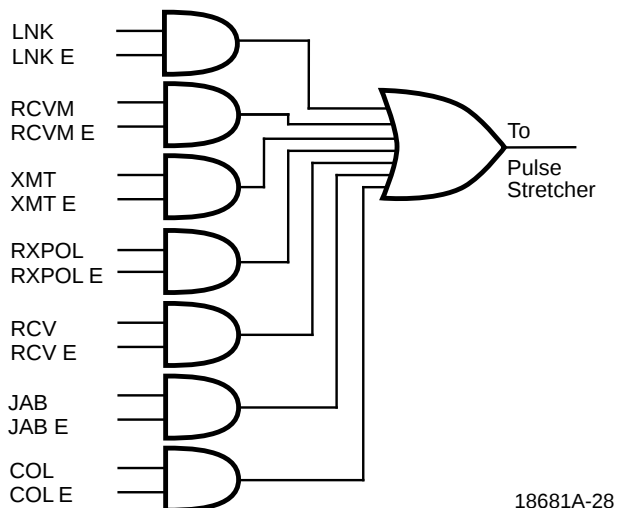
Figure 24. LED Control Logic
