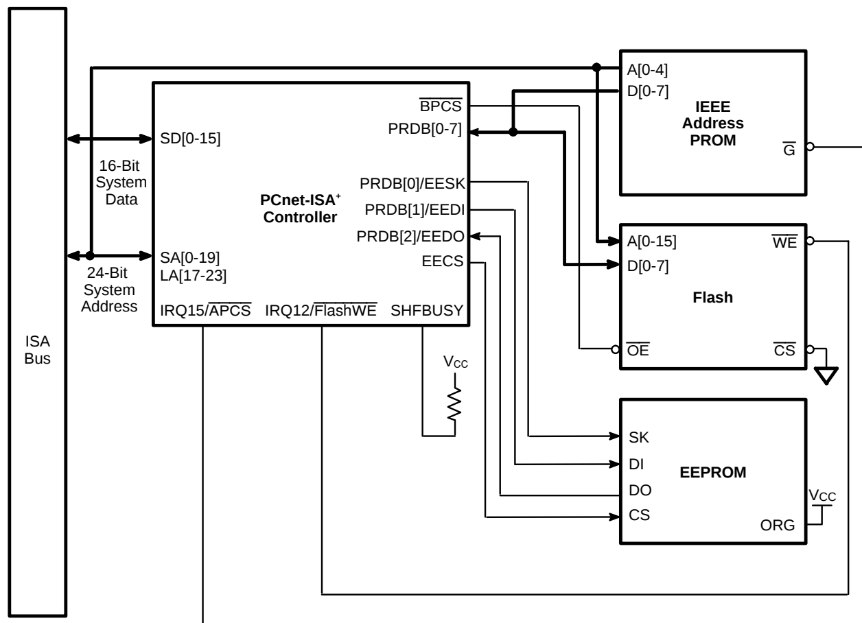
Bus Master Block Diagram Plug and Play Compatible with Flash Support
