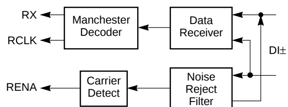
Figure 4. Receiver
