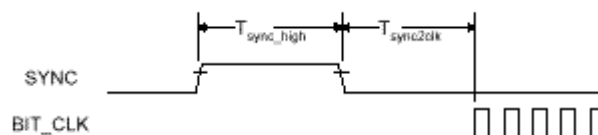
Warm reset timing diagram
