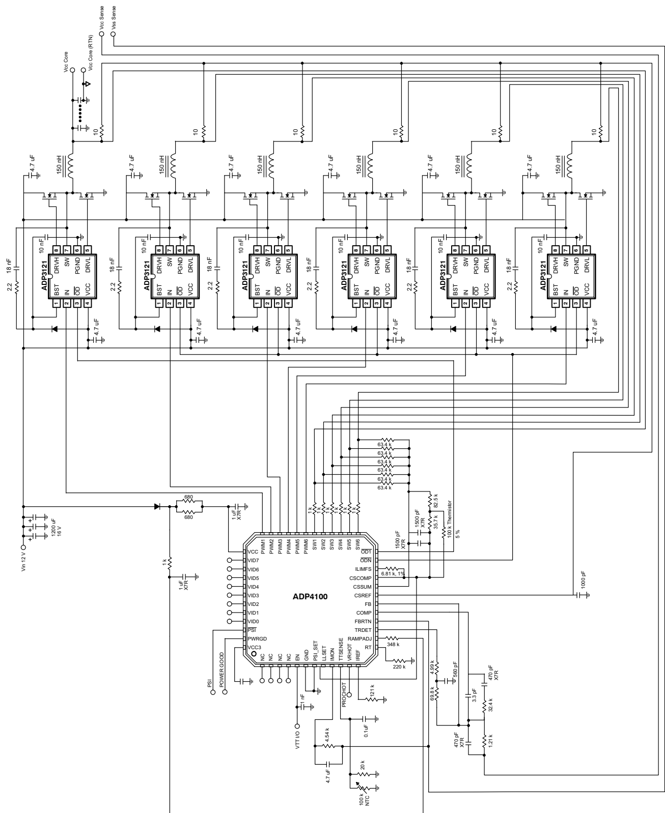
Figure 2. Application Schematic
