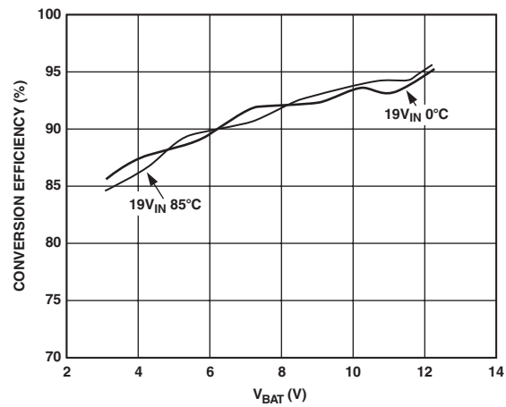
TPC 15. Conversion Efficiency vs. Battery Voltage at Given Temperatures
