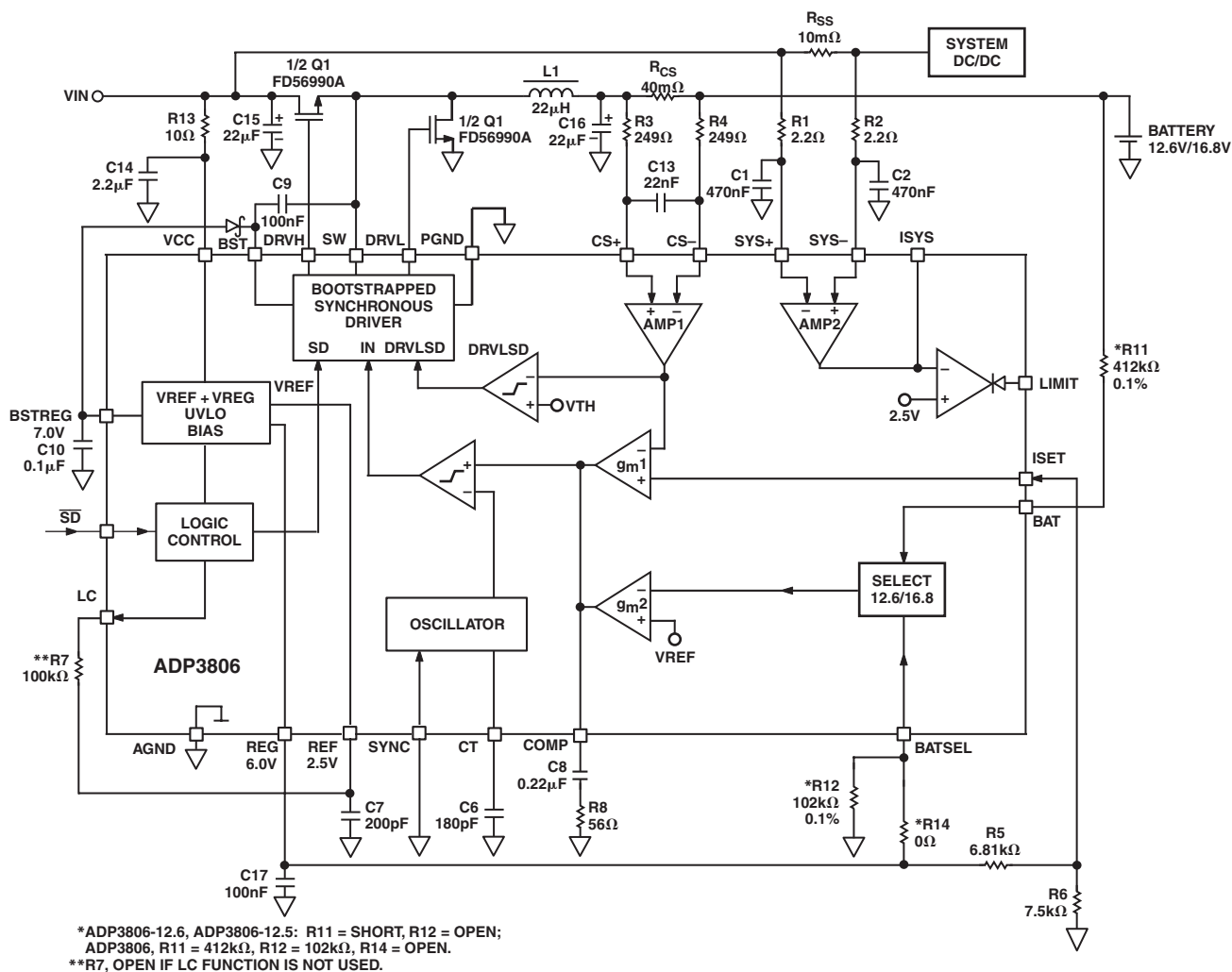
Figure 1. Typical Application
