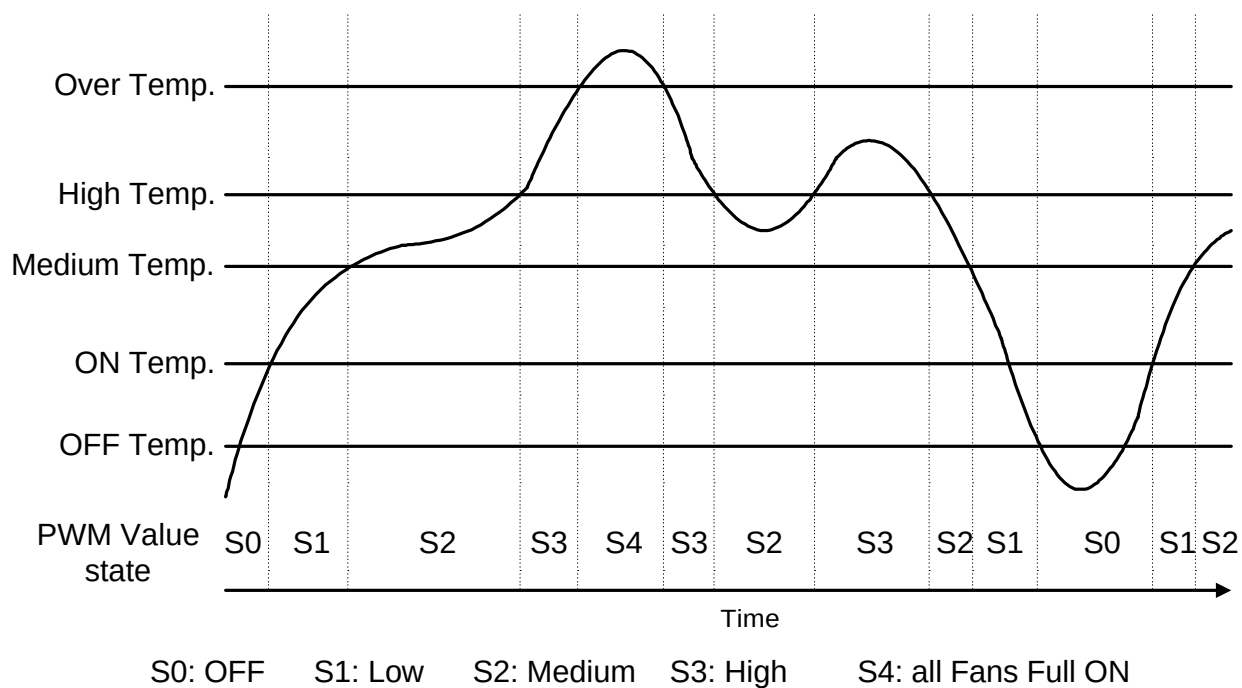
Figure 10-1. SmartGuardian Automatic Mode
