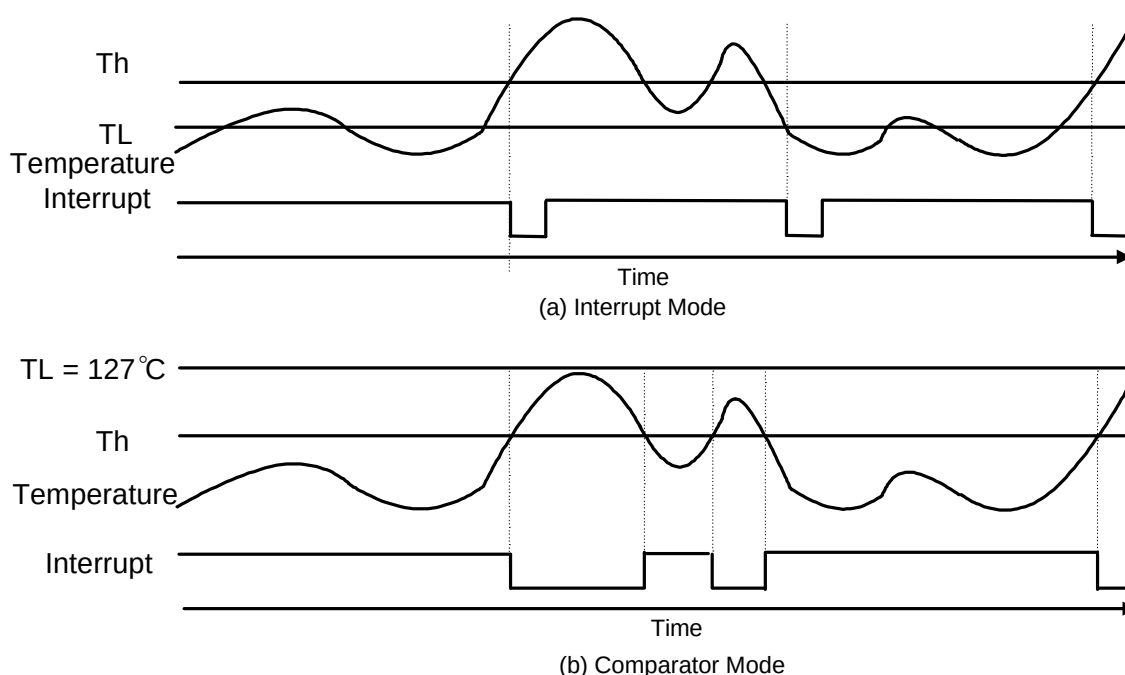
Figure 10-1. Temperature Interrupt Response Diagram
