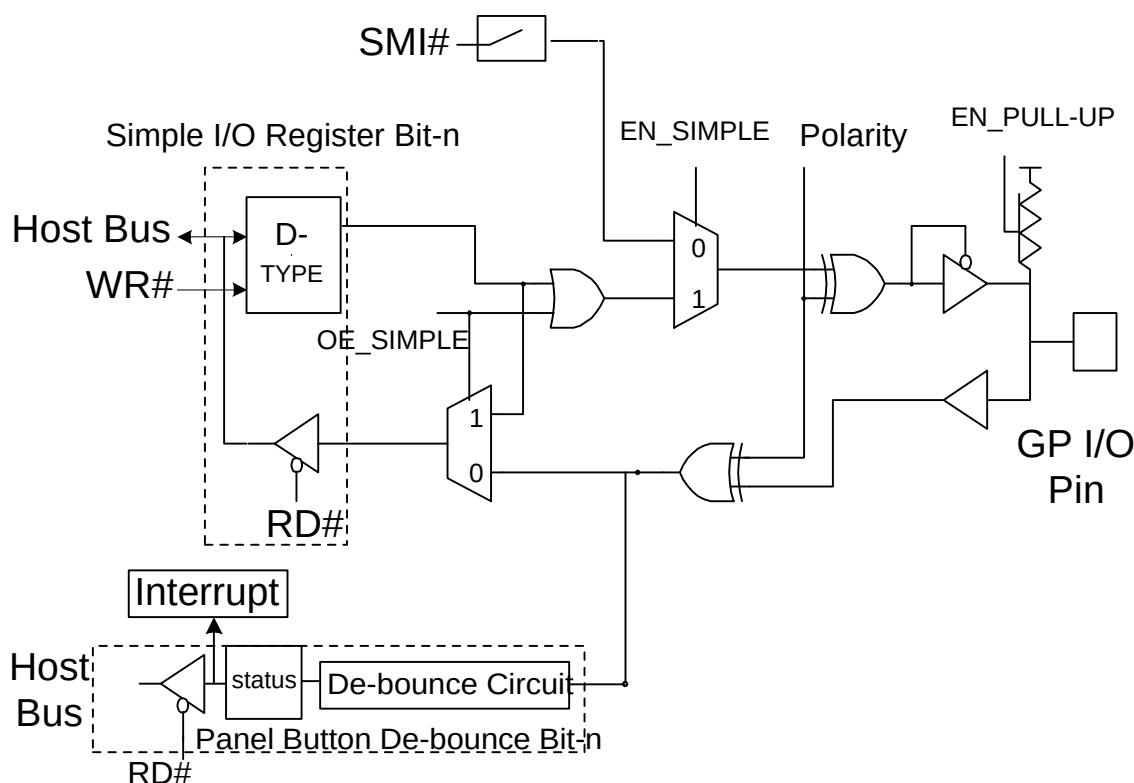
Figure 10-1. General Logic of GPIO Function
