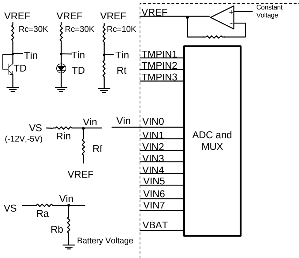
Figure 10-1. Application Example Resistor should provide approximately 2V at the Analog Inputs
