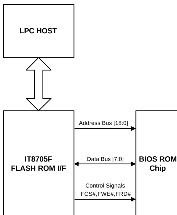
Figure 10-8. FLASH ROM Interface Diagram
