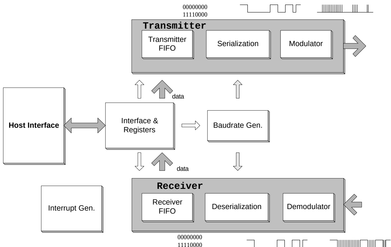
Figure 10-7. CIR Block Diagram
