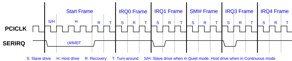
Figure 10-1. Start Frame Timing
