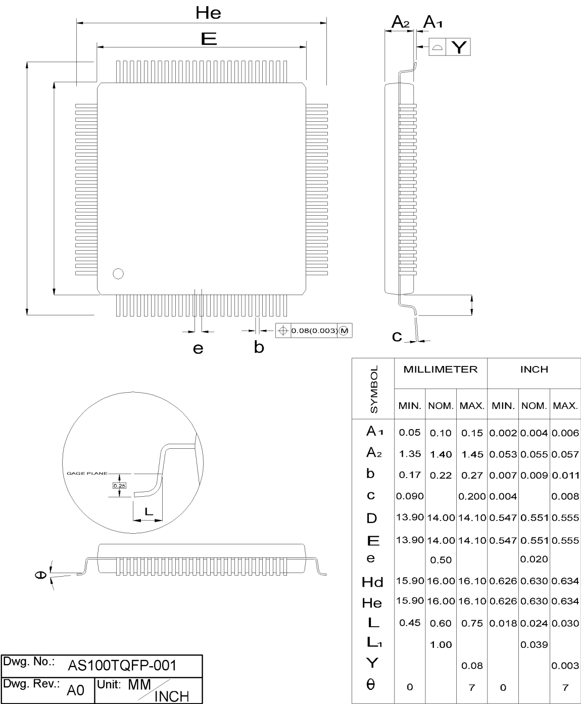
Figure 3. 100-Pin Low-Profile Quad Flat Pack (LQFP)
