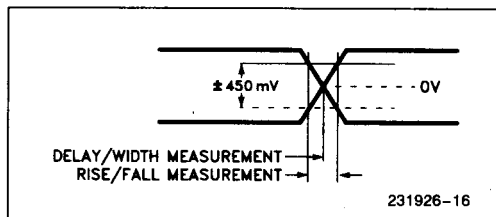
Figure 10A. Voltage Levels for \overline{TRMT}/\overline{TRMT} Output-Timing Measurements
