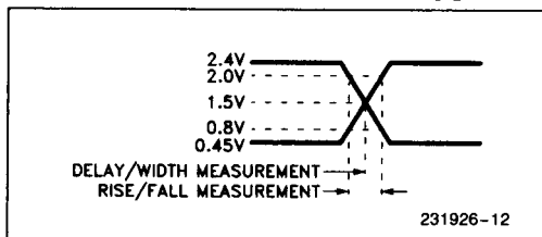
Figure 7. TTL Input Voltage Levels for Timing Measurements ( \overline{TEN} , \overline{TXD} , \overline{LPBK}/\overline{WDTD} ).
