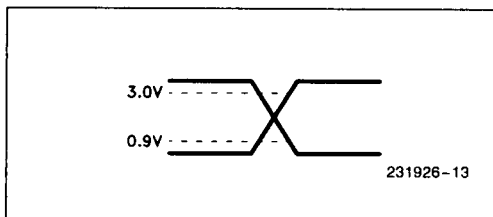
Figure 8. Voltage Levels for MOS Level Output-Timing Measurements ( \overline{TXC} , \overline{RXC} , \overline{CRS} , \overline{CDT} , and \overline{RXD} ).
