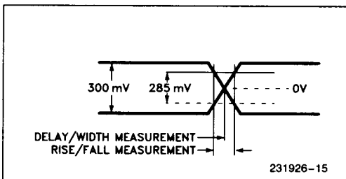
Figure 10. Voltage Levels for Differential-Input Timing Measurements ( \overline{RCV}/\overline{RCV} and \overline{CLSN}/\overline{CLSN} ).
