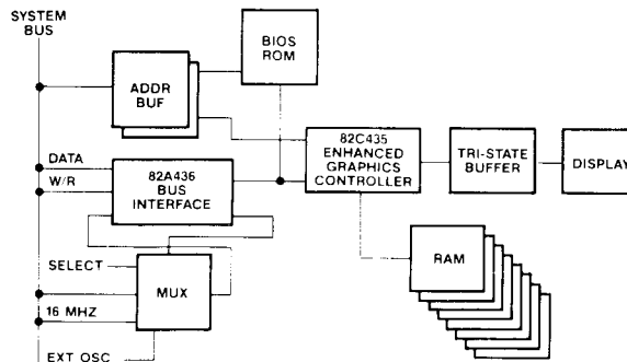
82C435/82A436 EGA System Diagram
