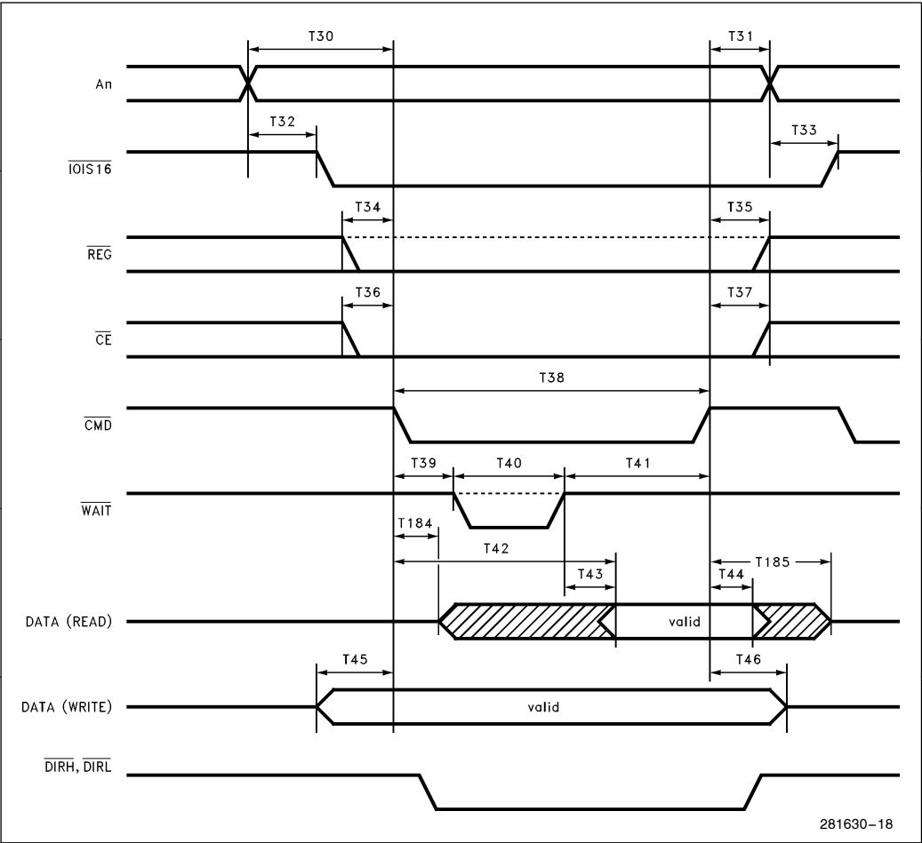
Figure 11-8. PCMCIA Cycle
