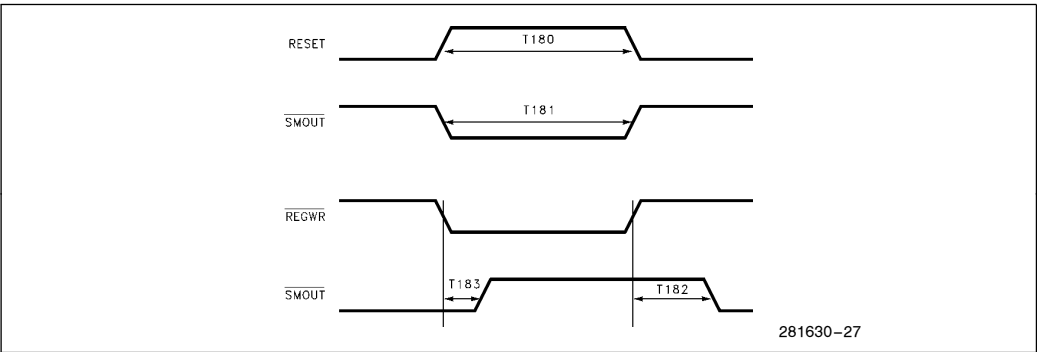
Figure 11-17. \overline{\text{SMOUT}} Timing
