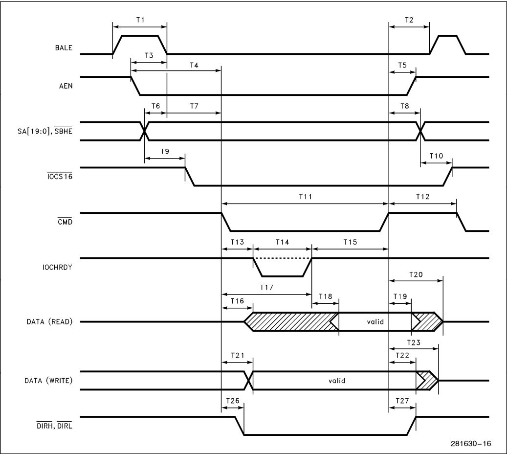
Figure 11-6. ISA-Compatible Cycle
