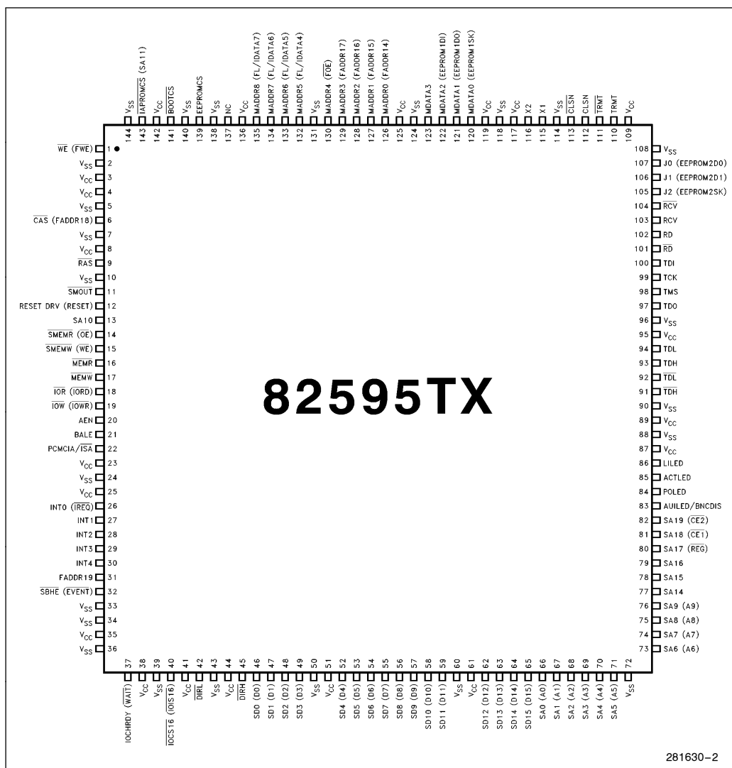
Figure 2. 82595TX Pinout
