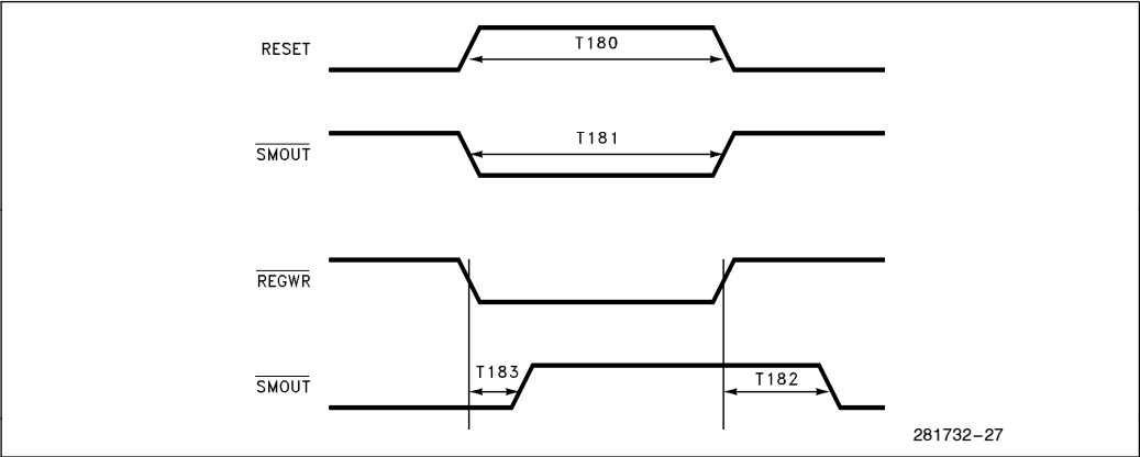
Figure 11-14. \overline{\text{SMOUT}} Timing
