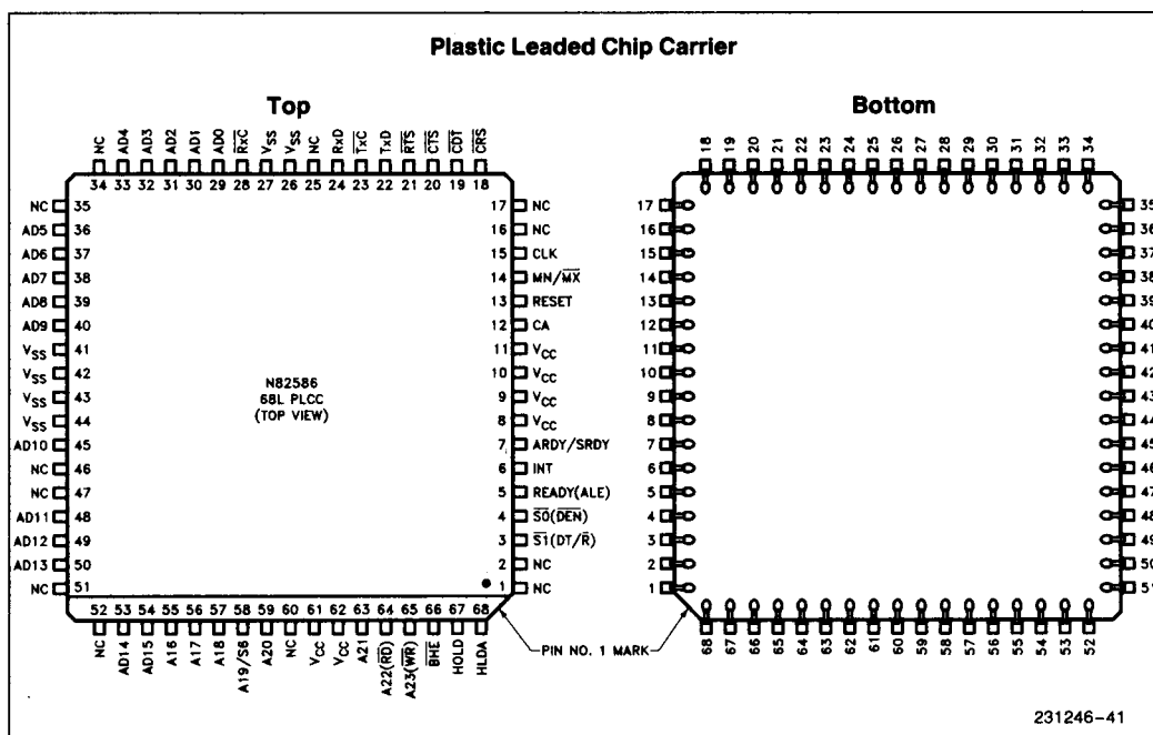
Figure 2. 82586 Pinout Diagrams
