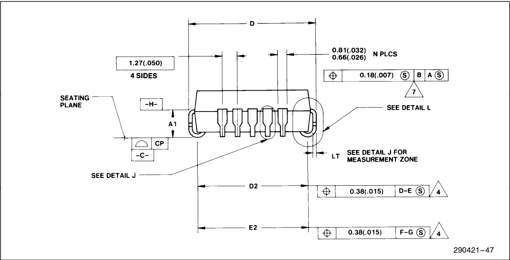
Figure 47. Terminal Details
