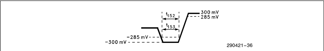
Figure 37. AUI Noise Filter Timings
