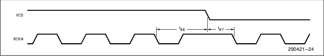
Figure 25. Receive Timings (Fujitsu—End of Frame)
