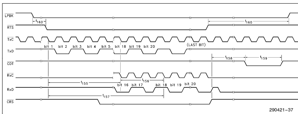
Figure 38. Loopback Timings
