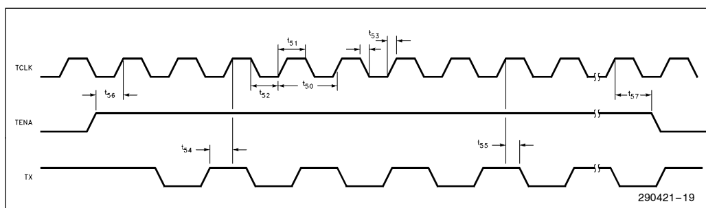
Figure 20. Transmit Timings (AMD)
