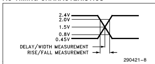
Figure 9. MOS Input Voltage Levels (TTL Compatible) for Timing Measurements (Tx D , RTS, TPE/AUI, A PORT , APOL/XSQ, LID, LPBK, JABD, TEST, and RESET).
