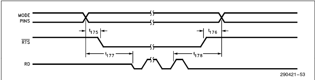
Figure 41. Mode Timings
