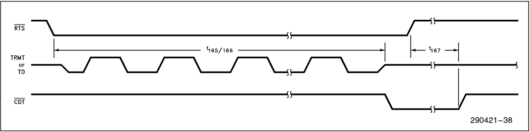
Figure 39. Jabber Timings
