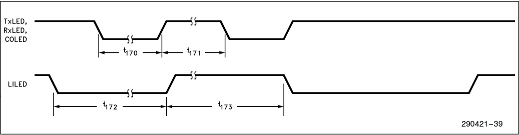
Figure 40. LED Timings
