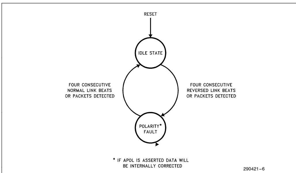
Figure 7. Polarity Fault State Diagram
