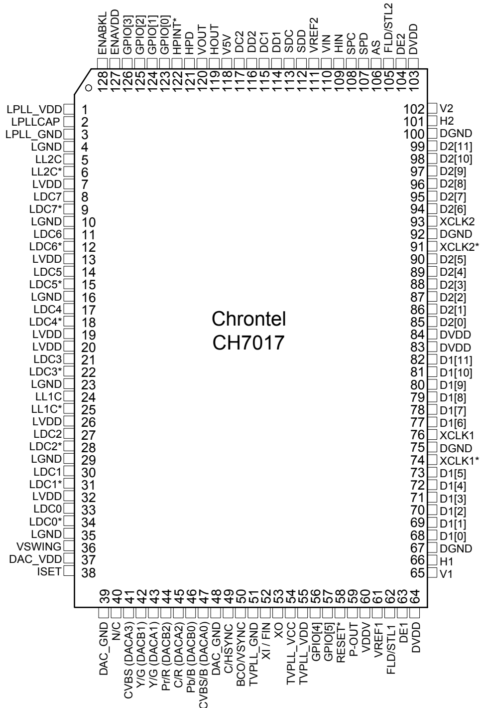
Figure 2: CH7017 128 Pin LQFP Package (Top View)
