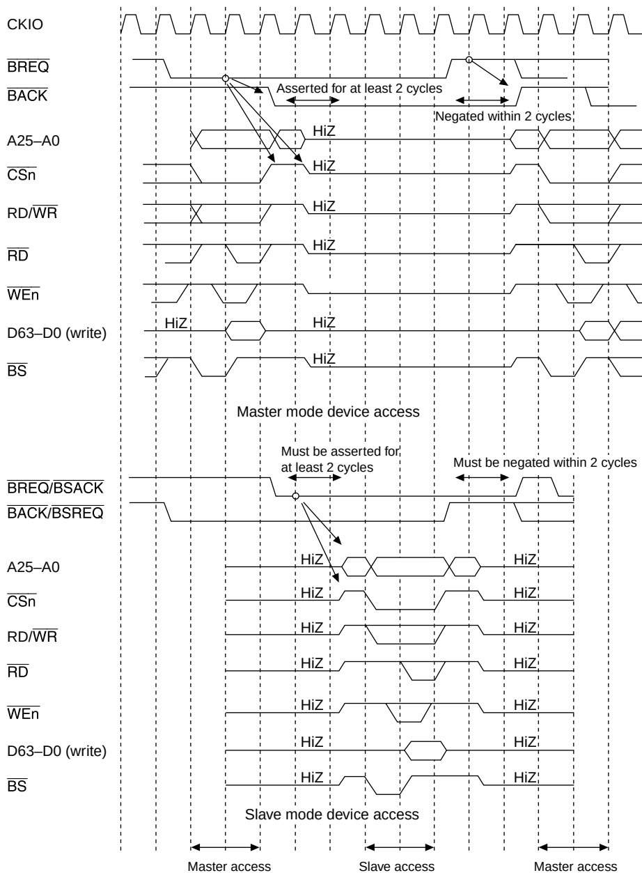
Figure 13.78 Arbitration Sequence
