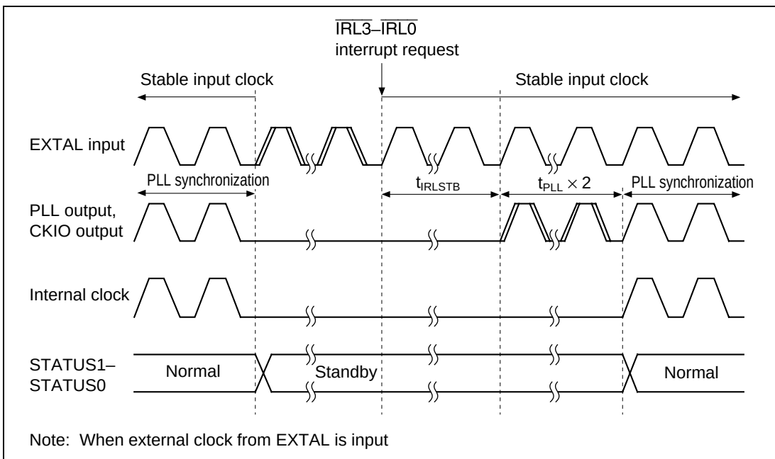
Figure 22.10 PLL Synchronization Settling Time in Case of IRL Interrupt
