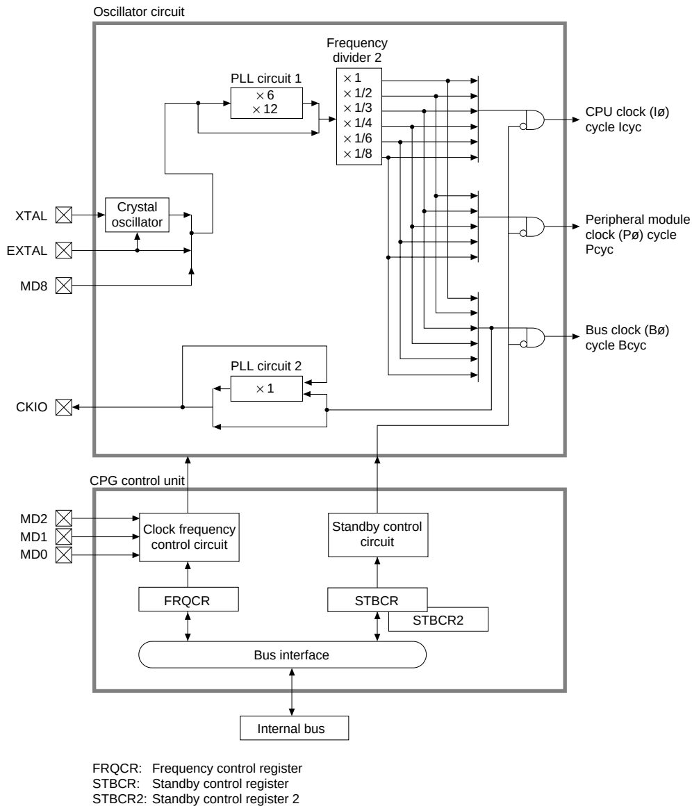
Figure 10.1 (2) Block Diagram of CPG (SH7750R)
