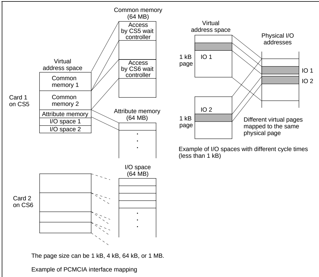
Figure 13.52 PCMCIA Space Allocation
