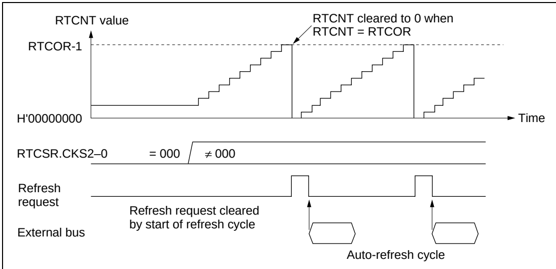
Figure 13.39 Auto-Refresh Operation
