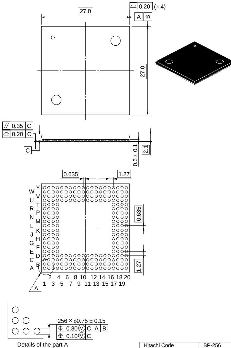
Figure B.1 Package Dimensions (256-Pin BGA) (SH7750 and SH7750S)
