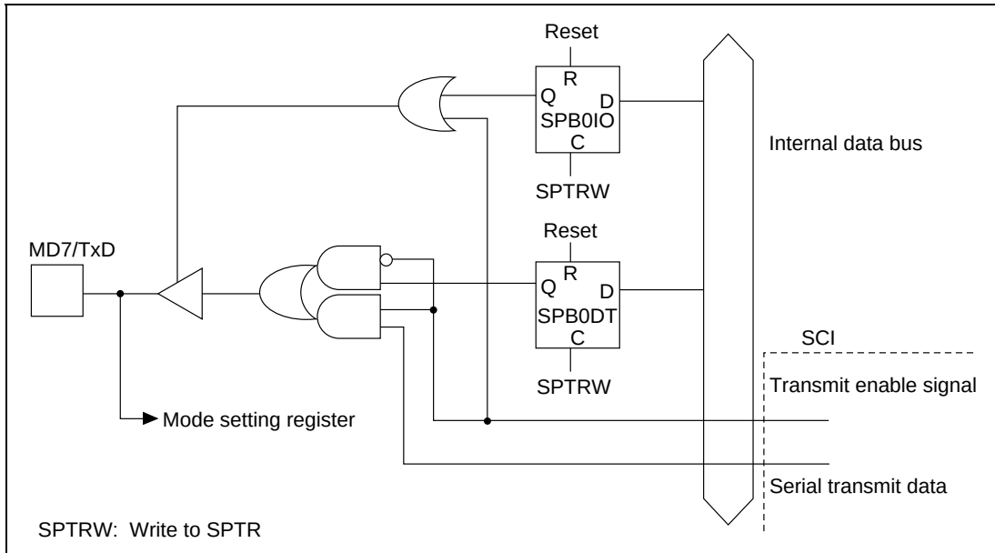
Figure 18.4 MD7/TxD Pin
