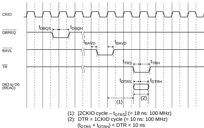
Figure 22.66(b) \overline{\text{DBREQ}}/\text{TR} Input Timing and \overline{\text{BAVL}} Output Timing
