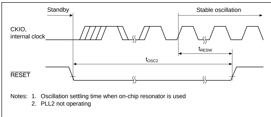
Figure 22.4 Standby Return Oscillation Settling Time (Return by RESET)
