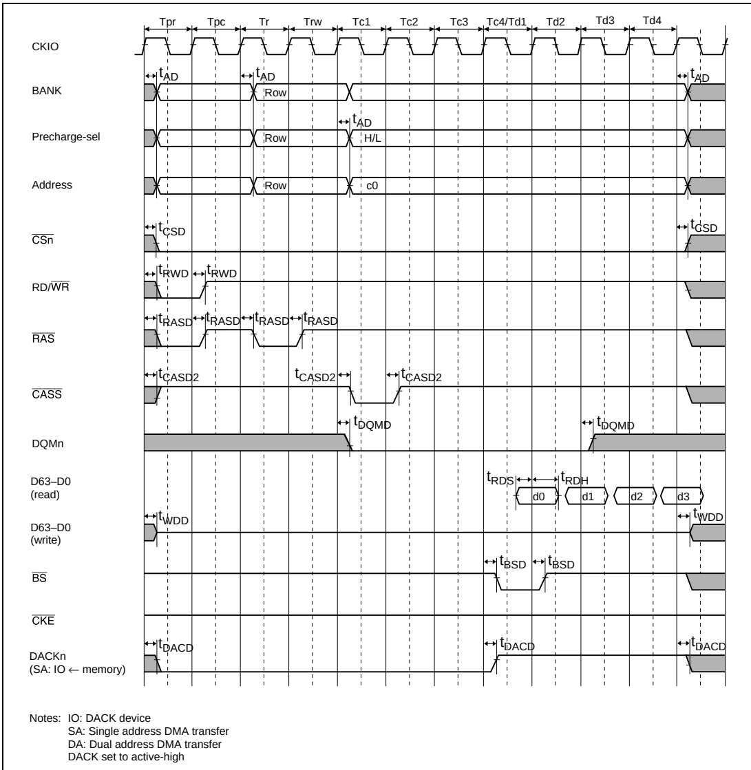
Figure 22.26 Synchronous DRAM Normal Read Bus Cycle: PRE + ACT + READ Commands, Burst (RCD[1:0] = 01, TPC[2:0] = 001, CAS Latency = 3)
