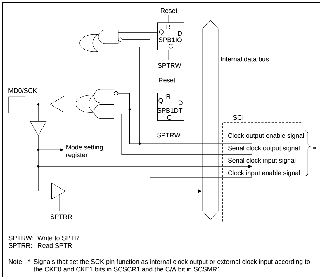
Figure 18.3 MD0/SCK Pin
