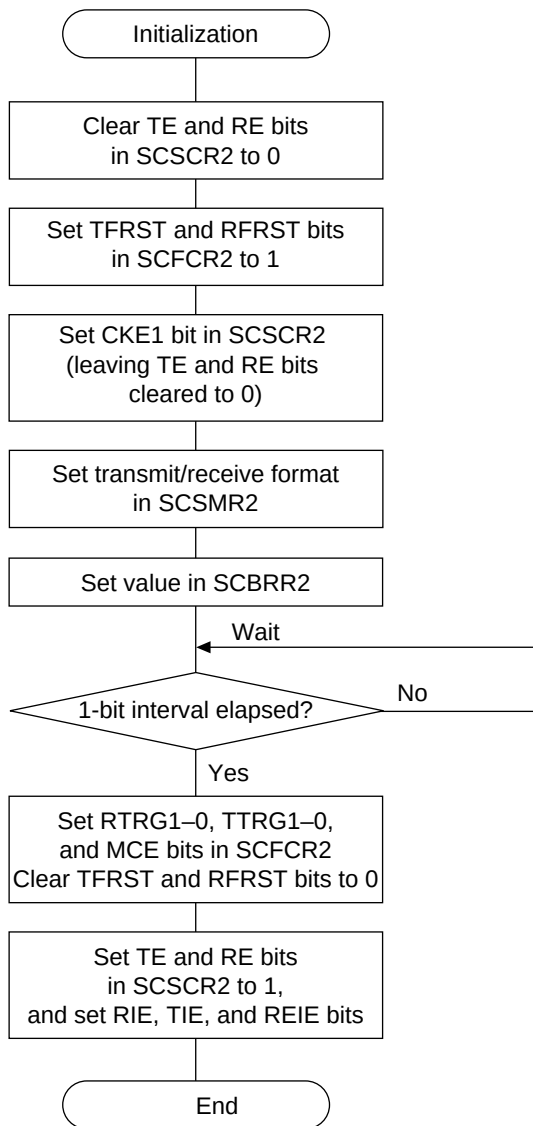
Figure 16.6 Sample SCIF Initialization Flowchart
