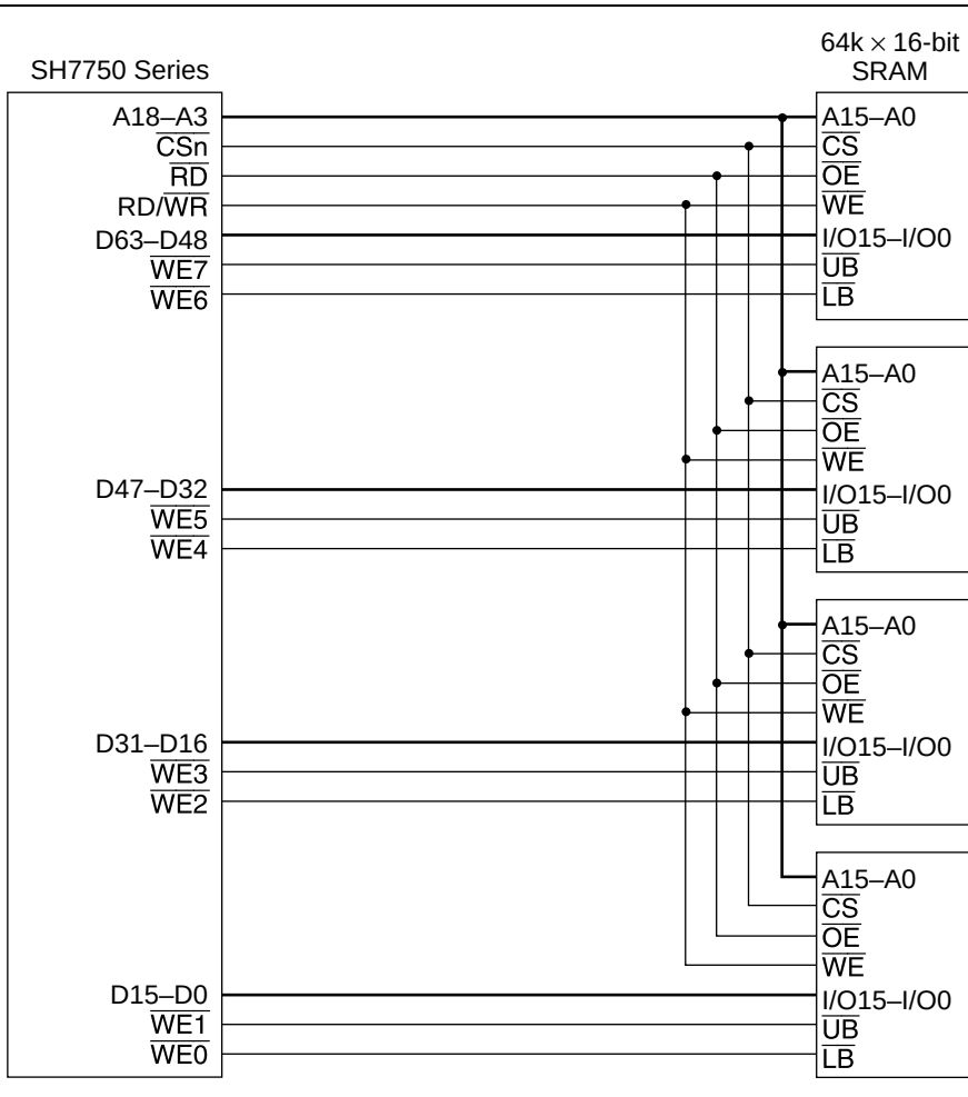
Figure 13.73 Example of 64-Bit Data Width Byte Control SRAM
